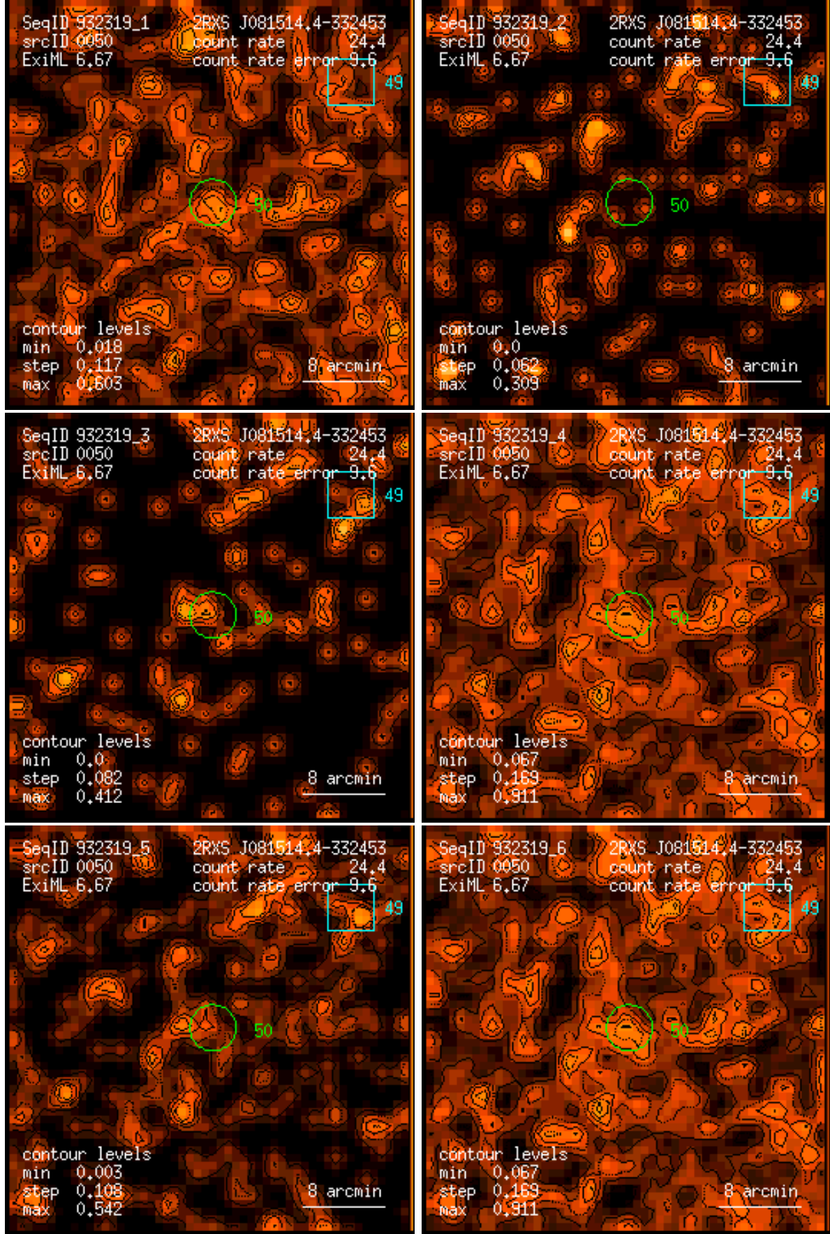
Figure 50: RASS 932319: detection 0050: band rate images, Gaussian filter: (1) PSPC channels 11 – 41, (2) 52 – 90, (3) 91 – 201, (4) 11 – 235, (5) 52 – 201, (6) 11 – 201. Broad band rates in counts/ks. Band rate contour levels in counts/ks/arcmin 2 .
