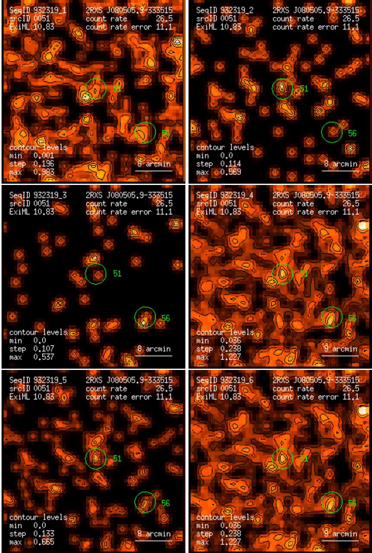
Figure 51: RASS 932319: detection 0051: band rate images, Gaussian filter: (1) PSPC channels 11 – 41, (2) 52 – 90, (3) 91 – 201, (4) 11 – 235, (5) 52 – 201, (6) 11 – 201. Broad band rates in counts/ks. Band rate contour levels in counts/ks/arcmin 2 .
