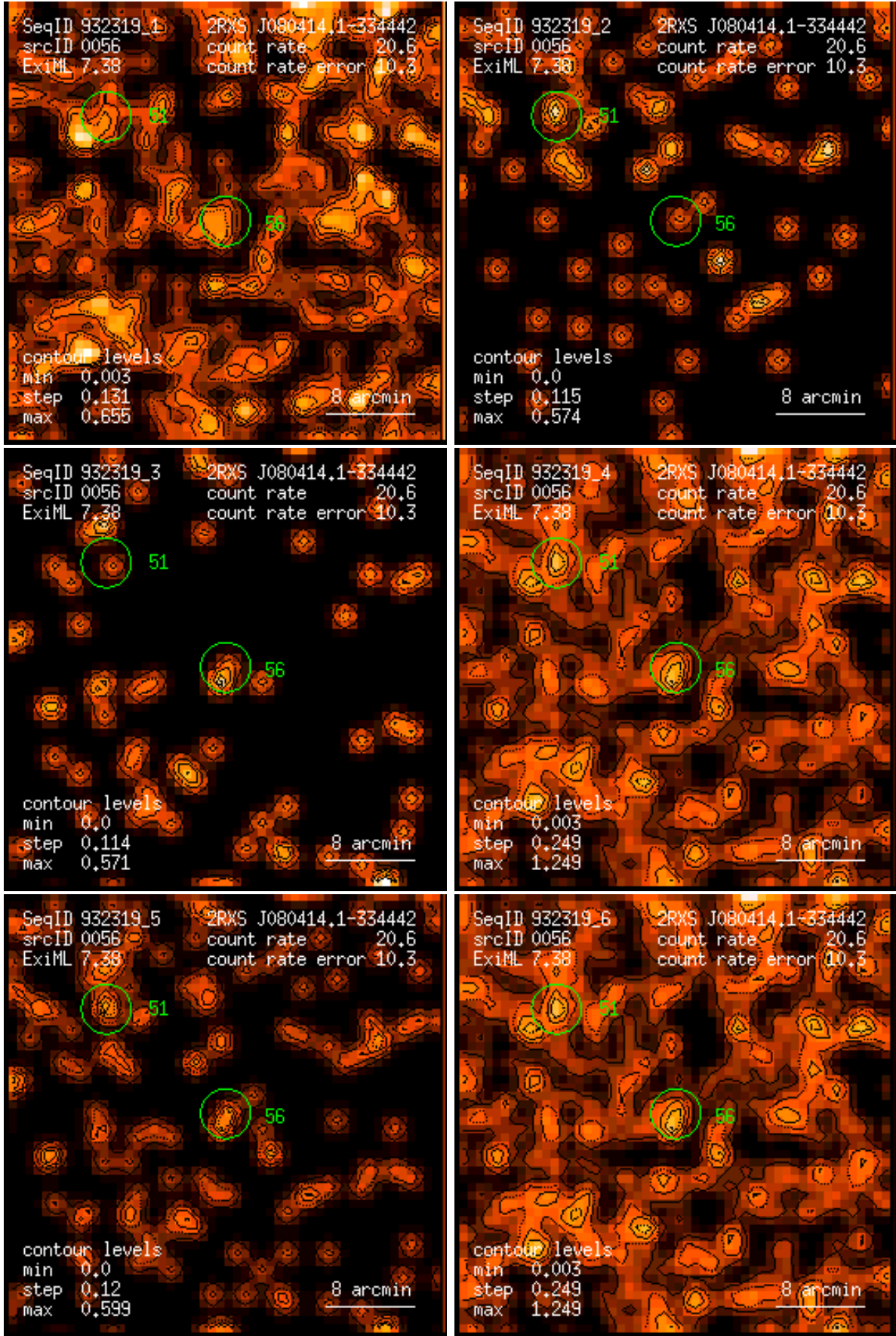
Figure 56: RASS 932319: detection 0056: band rate images, Gaussian filter: (1) PSPC channels 11 – 41, (2) 52 – 90, (3) 91 – 201, (4) 11 – 235, (5) 52 – 201, (6) 11 – 201. Broad band rates in counts/ks. Band rate contour levels in counts/ks/arcmin 2 .
