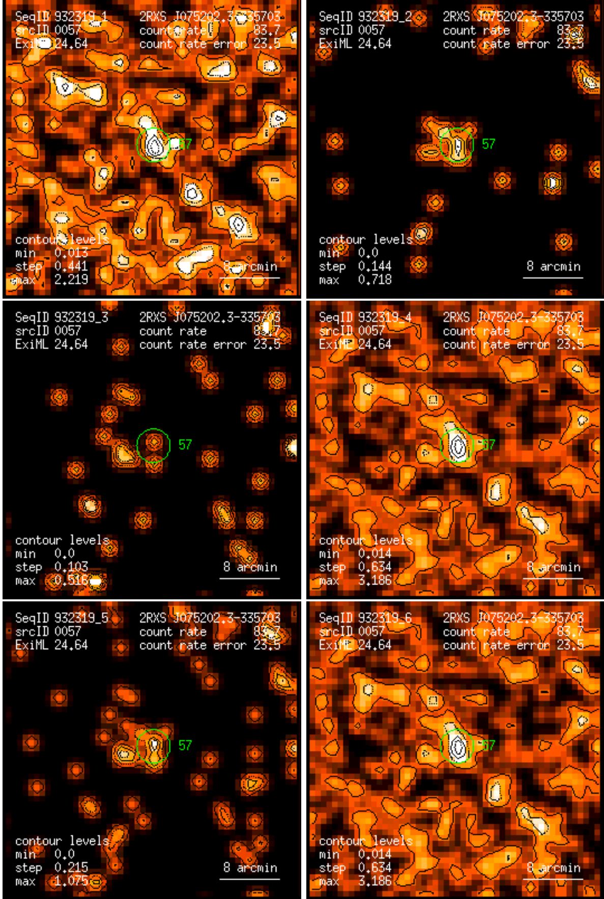
Figure 57: RASS 932319: detection 0057: band rate images, Gaussian filter: (1) PSPC channels 11 – 41, (2) 52 – 90, (3) 91 – 201, (4) 11 – 235, (5) 52 – 201, (6) 11 – 201. Broad band rates in counts/ks. Band rate contour levels in counts/ks/arcmin 2 .
