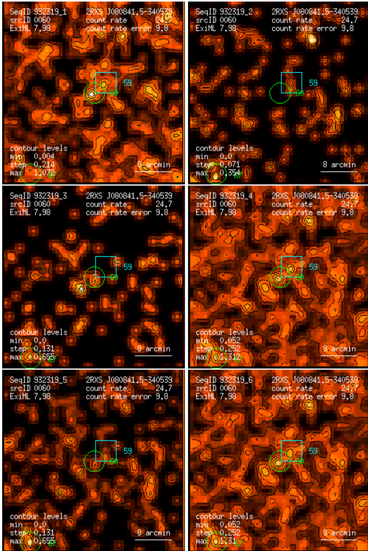
Figure 60: RASS 932319: detection 0060: band rate images, Gaussian filter: (1) PSPC channels 11 – 41, (2) 52 – 90, (3) 91 – 201, (4) 11 – 235, (5) 52 – 201, (6) 11 – 201. Broad band rates in counts/ks. Band rate contour levels in counts/ks/arcmin 2 .
