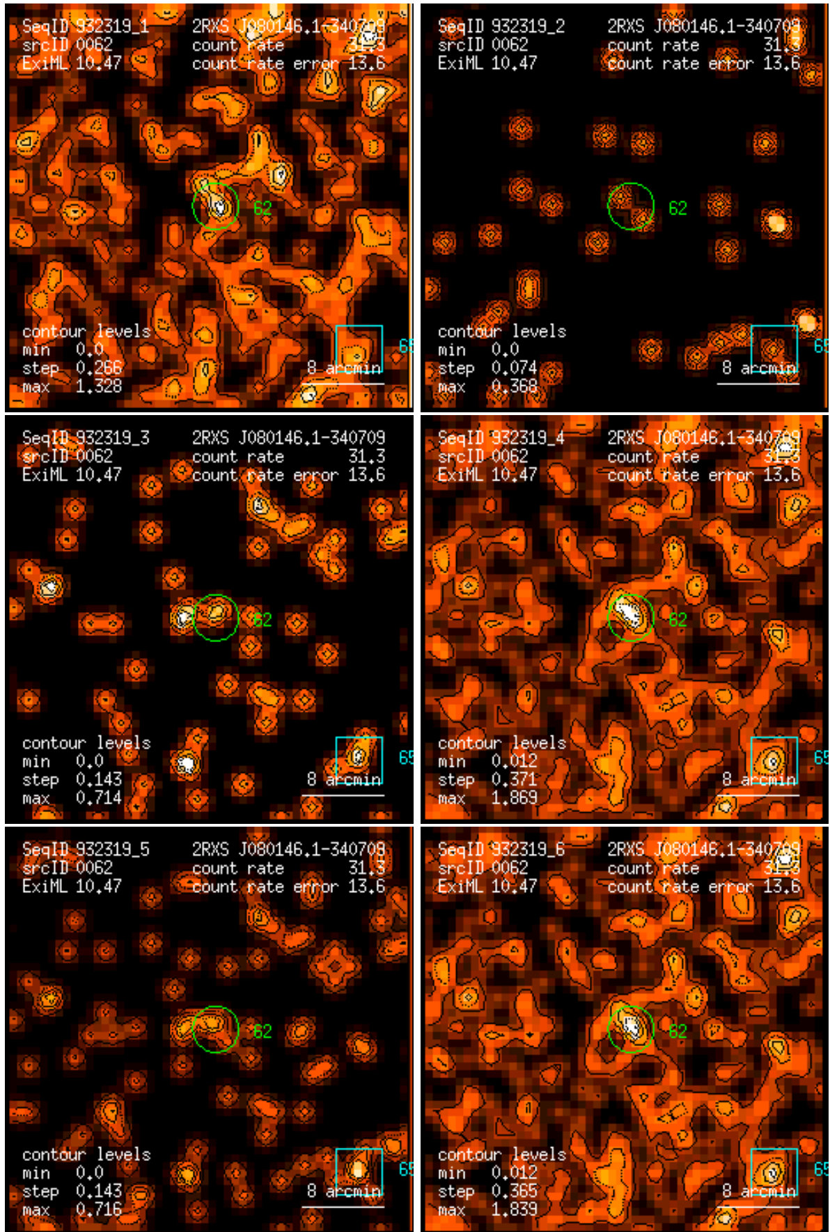
Figure 62: RASS 932319: detection 0062: band rate images, Gaussian filter: (1) PSPC channels 11 – 41, (2) 52 – 90, (3) 91 – 201, (4) 11 – 235, (5) 52 – 201, (6) 11 – 201. Broad band rates in counts/ks. Band rate contour levels in counts/ks/arcmin 2 .
