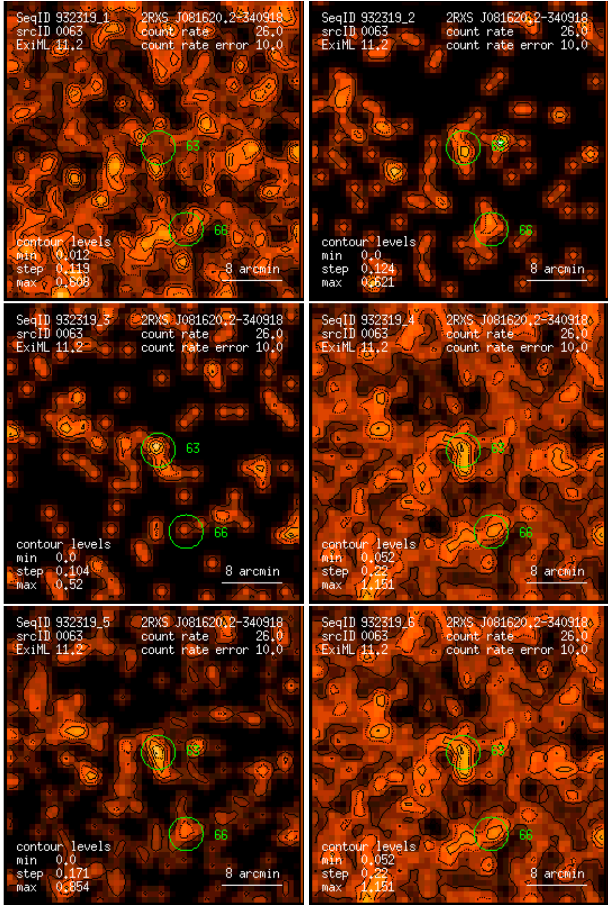
Figure 63: RASS 932319: detection 0063: band rate images, Gaussian filter: (1) PSPC channels 11 – 41, (2) 52 – 90, (3) 91 – 201, (4) 11 – 235, (5) 52 – 201, (6) 11 – 201. Broad band rates in counts/ks. Band rate contour levels in counts/ks/arcmin 2 .
