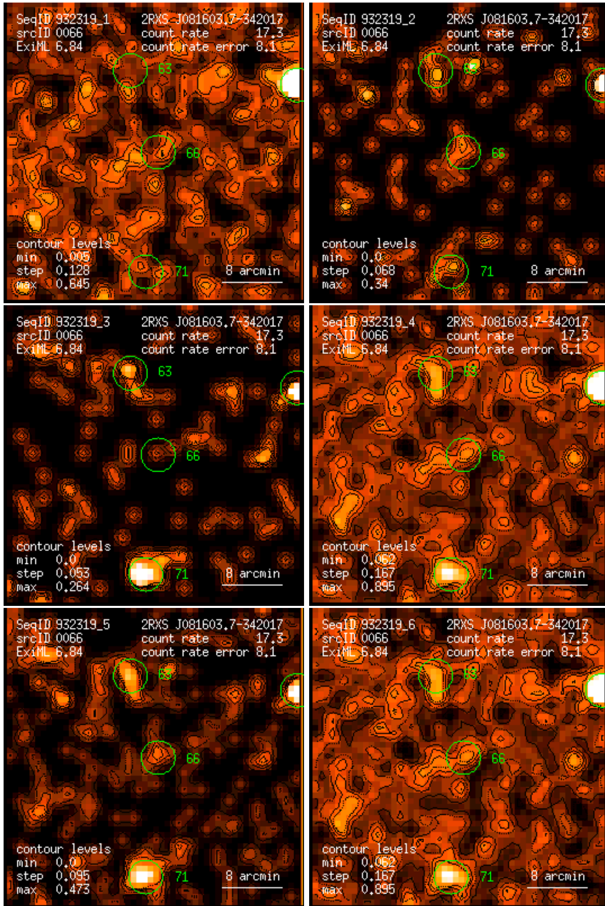
Figure 66: RASS 932319: detection 0066: band rate images, Gaussian filter: (1) PSPC channels 11 – 41, (2) 52 – 90, (3) 91 – 201, (4) 11 – 235, (5) 52 – 201, (6) 11 – 201. Broad band rates in counts/ks. Band rate contour levels in counts/ks/arcmin 2 .
