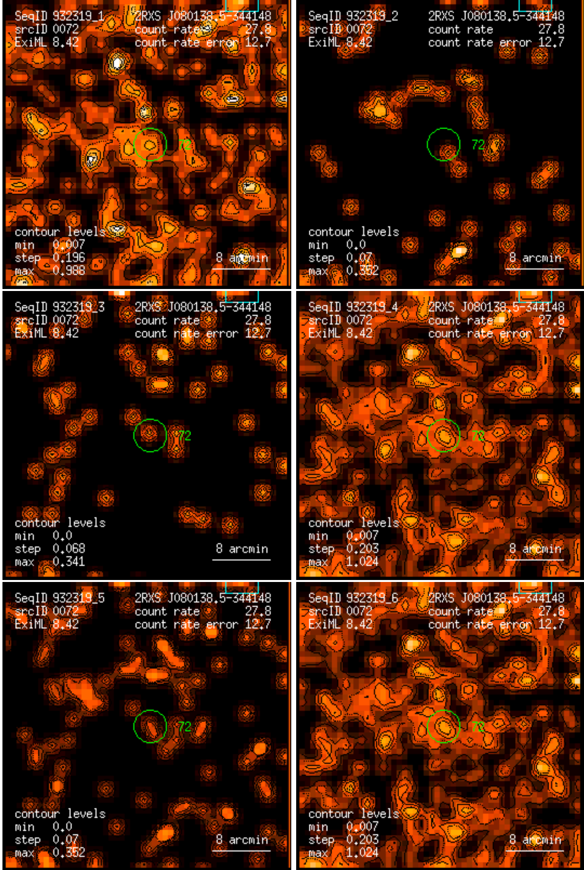
Figure 72: RASS 932319: detection 0072: band rate images, Gaussian filter: (1) PSPC channels 11 – 41, (2) 52 – 90, (3) 91 – 201, (4) 11 – 235, (5) 52 – 201, (6) 11 – 201. Broad band rates in counts/ks. Band rate contour levels in counts/ks/arcmin 2 .
