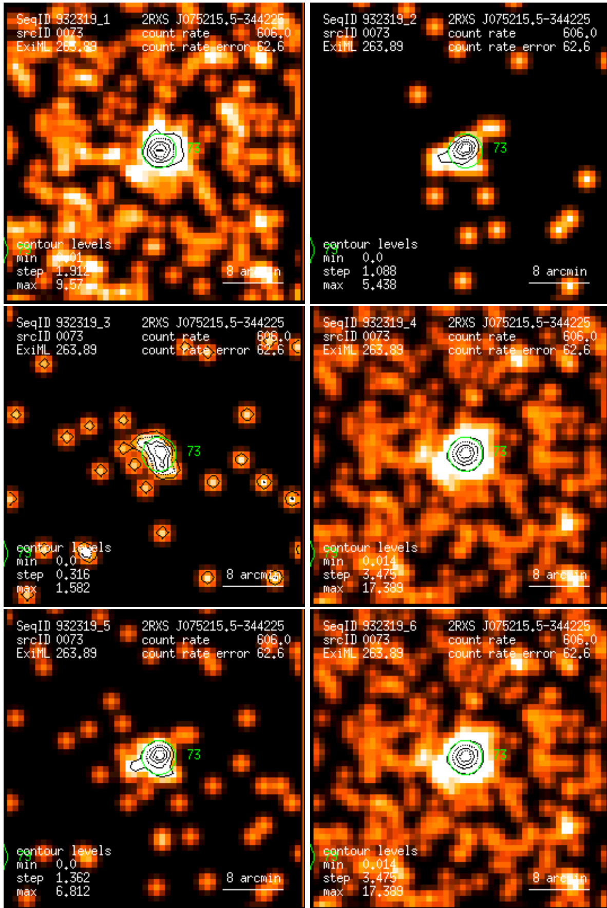
Figure 73: RASS 932319: detection 0073: band rate images, Gaussian filter: (1) PSPC channels 11 – 41, (2) 52 – 90, (3) 91 – 201, (4) 11 – 235, (5) 52 – 201, (6) 11 – 201. Broad band rates in counts/ks. Band rate contour levels in counts/ks/arcmin 2 .
