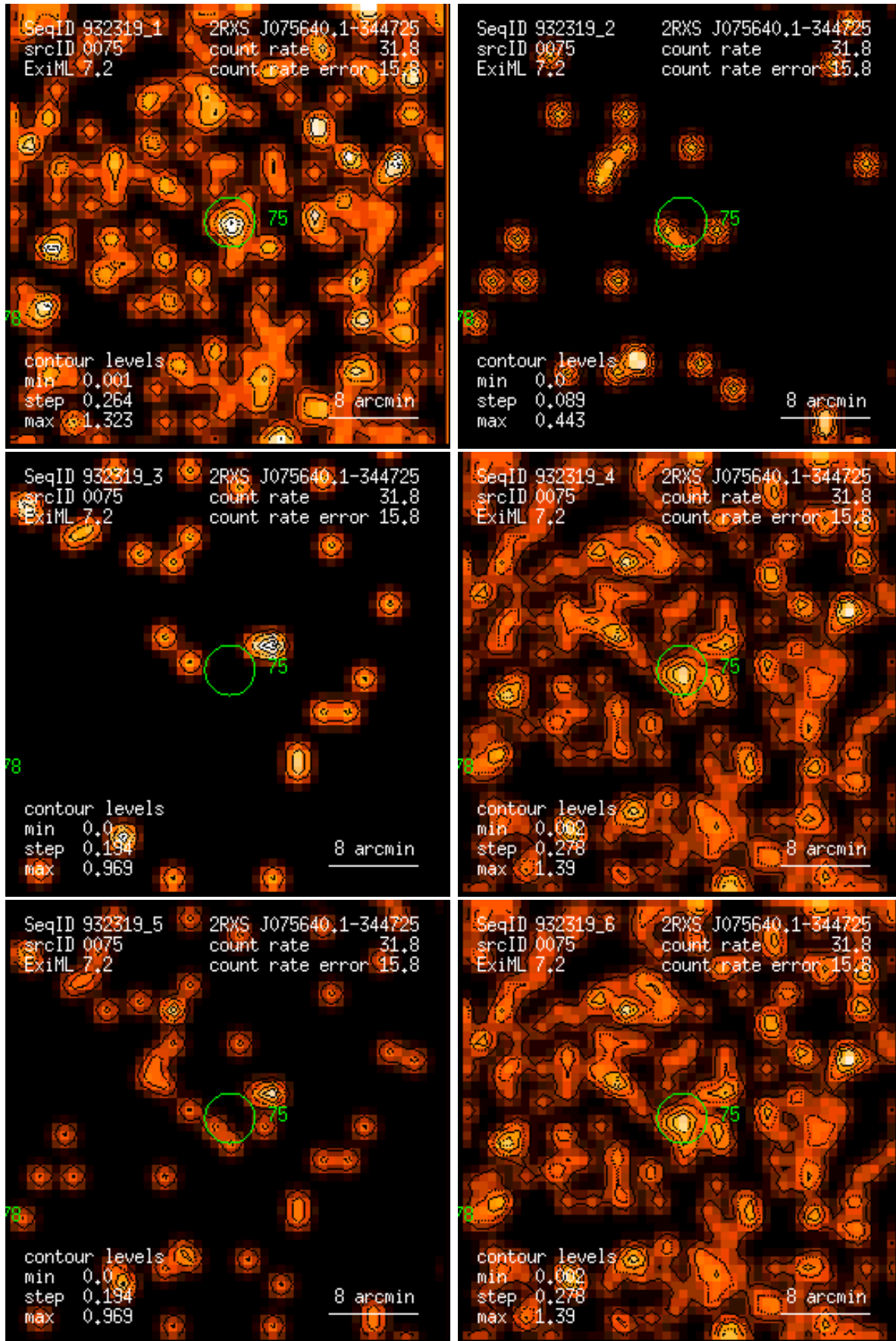
Figure 75: RASS 932319: detection 0075: band rate images, Gaussian filter: (1) PSPC channels 11 – 41, (2) 52 – 90, (3) 91 – 201, (4) 11 – 235, (5) 52 – 201, (6) 11 – 201. Broad band rates in counts/ks. Band rate contour levels in counts/ks/arcmin 2 .
