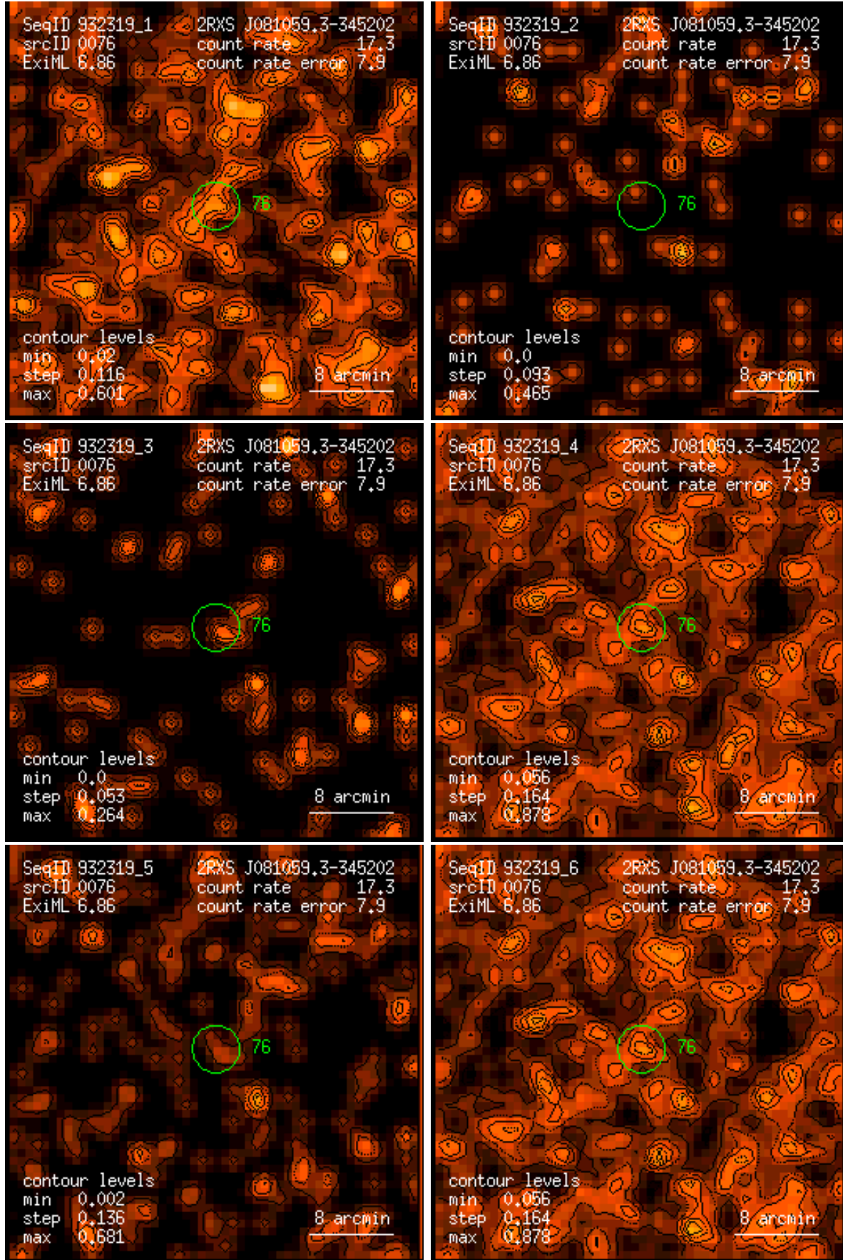
Figure 76: RASS 932319: detection 0076: band rate images, Gaussian filter: (1) PSPC channels 11 – 41, (2) 52 – 90, (3) 91 – 201, (4) 11 – 235, (5) 52 – 201, (6) 11 – 201. Broad band rates in counts/ks. Band rate contour levels in counts/ks/arcmin 2 .
