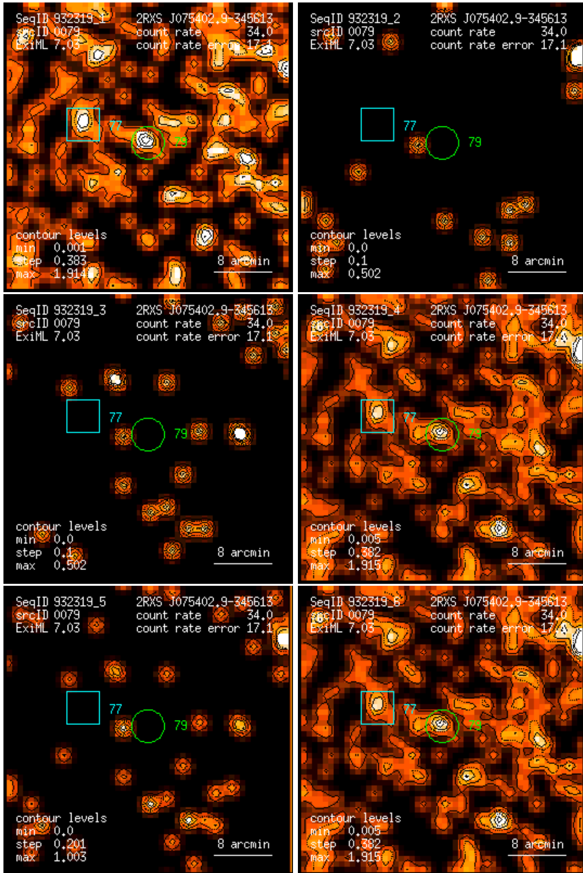
Figure 79: RASS 932319: detection 0079: band rate images, Gaussian filter: (1) PSPC channels 11 – 41, (2) 52 – 90, (3) 91 – 201, (4) 11 – 235, (5) 52 – 201, (6) 11 – 201. Broad band rates in counts/ks. Band rate contour levels in counts/ks/arcmin 2 .
