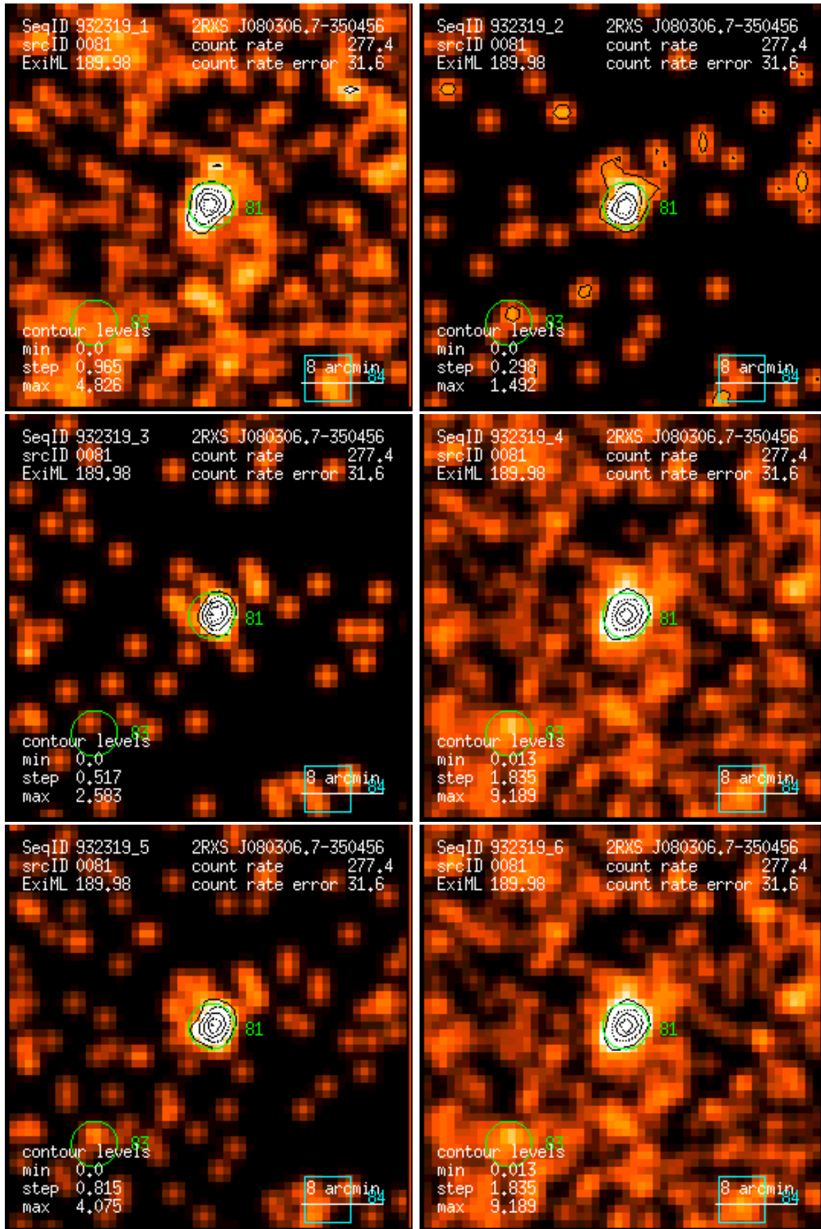
Figure 81: RASS 932319: detection 0081: band rate images, Gaussian filter: (1) PSPC channels 11 – 41, (2) 52 – 90, (3) 91 – 201, (4) 11 – 235, (5) 52 – 201, (6) 11 – 201. Broad band rates in counts/ks. Band rate contour levels in counts/ks/arcmin 2 .
