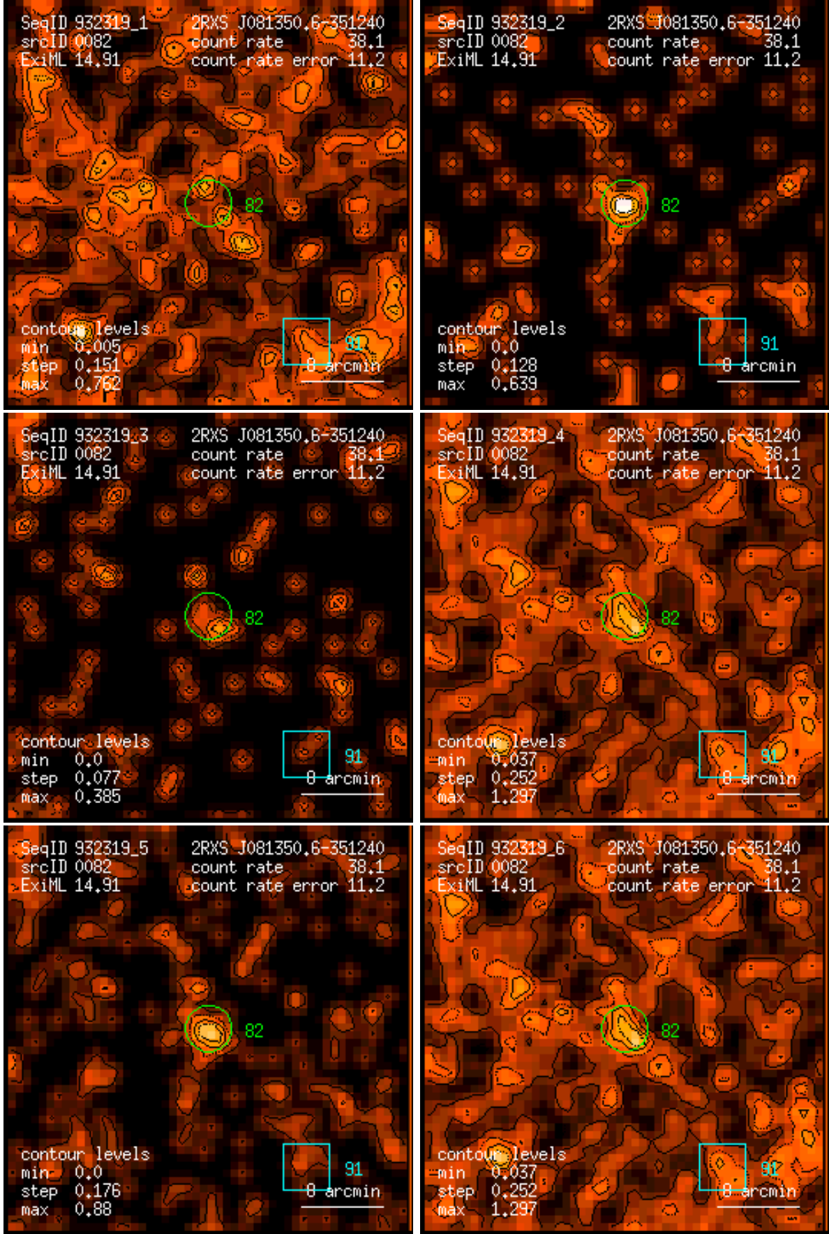
Figure 82: RASS 932319: detection 0082: band rate images, Gaussian filter: (1) PSPC channels 11 – 41, (2) 52 – 90, (3) 91 – 201, (4) 11 – 235, (5) 52 – 201, (6) 11 – 201. Broad band rates in counts/ks. Band rate contour levels in counts/ks/arcmin 2 .
