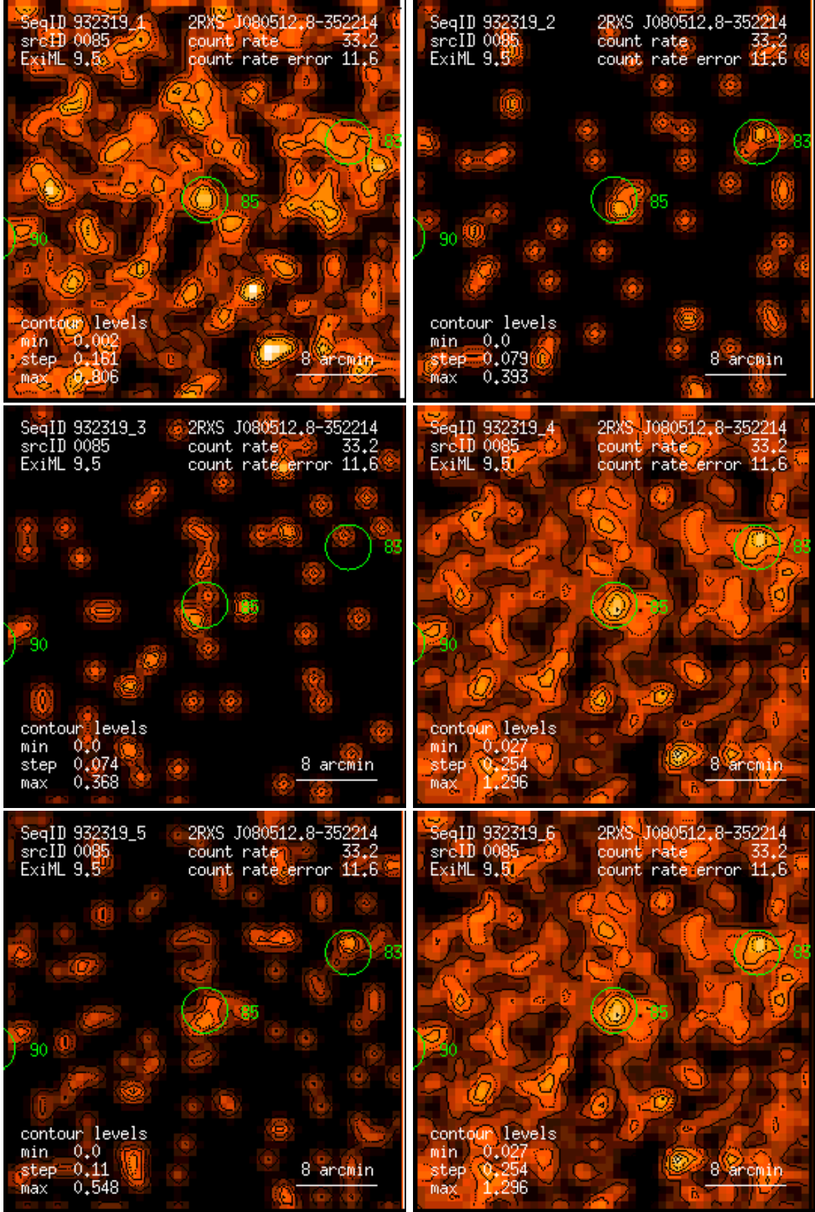
Figure 85: RASS 932319: detection 0085: band rate images, Gaussian filter: (1) PSPC channels 11 – 41, (2) 52 – 90, (3) 91 – 201, (4) 11 – 235, (5) 52 – 201, (6) 11 – 201. Broad band rates in counts/ks. Band rate contour levels in counts/ks/arcmin 2 .
