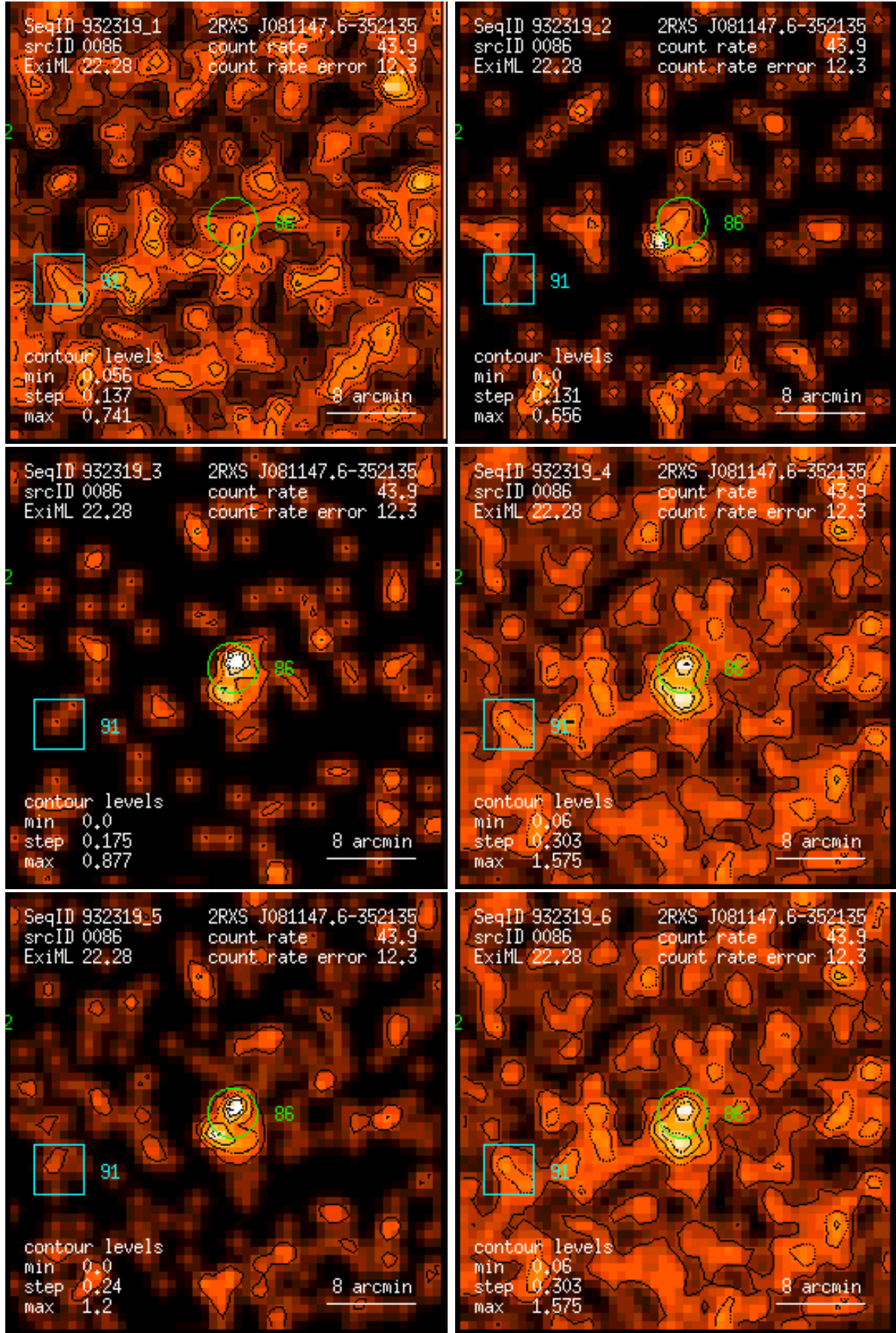
Figure 86: RASS 932319: detection 0086: band rate images, Gaussian filter: (1) PSPC channels 11 – 41, (2) 52 – 90, (3) 91 – 201, (4) 11 – 235, (5) 52 – 201, (6) 11 – 201. Broad band rates in counts/ks. Band rate contour levels in counts/ks/arcmin 2 .
