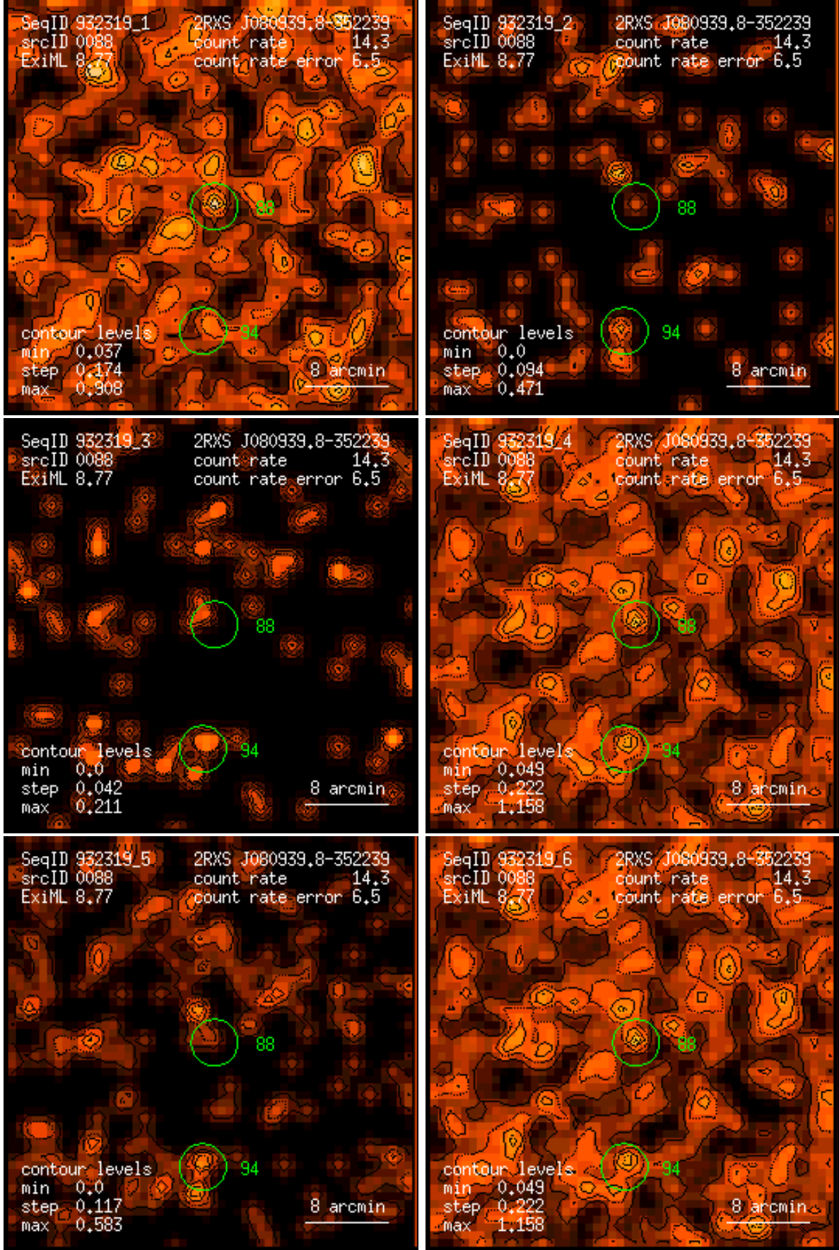
Figure 88: RASS 932319: detection 0088: band rate images, Gaussian filter: (1) PSPC channels 11 – 41, (2) 52 – 90, (3) 91 – 201, (4) 11 – 235, (5) 52 – 201, (6) 11 – 201. Broad band rates in counts/ks. Band rate contour levels in counts/ks/arcmin 2 .
