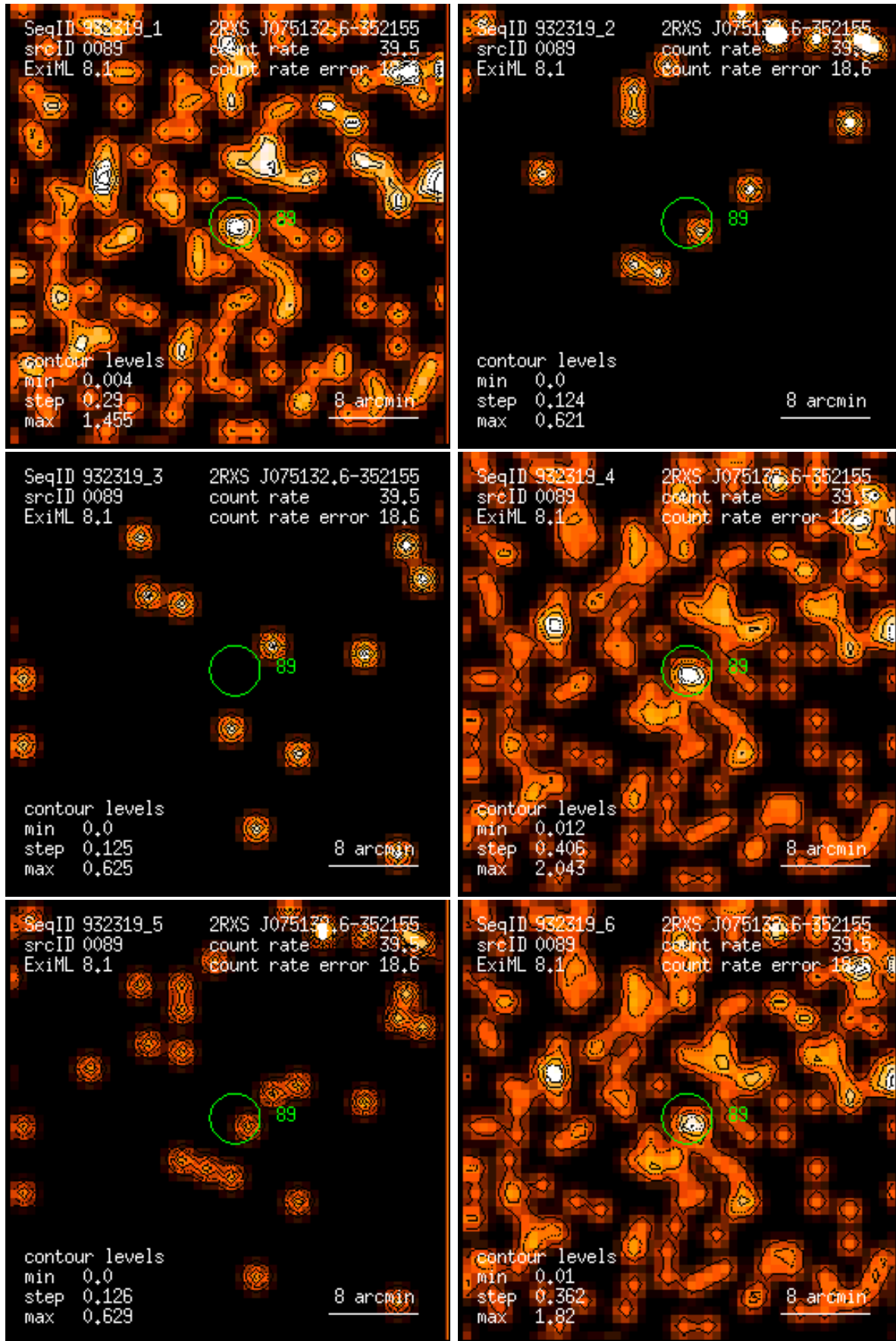
Figure 89: RASS 932319: detection 0089: band rate images, Gaussian filter: (1) PSPC channels 11 – 41, (2) 52 – 90, (3) 91 – 201, (4) 11 – 235, (5) 52 – 201, (6) 11 – 201. Broad band rates in counts/ks. Band rate contour levels in counts/ks/arcmin 2 .
