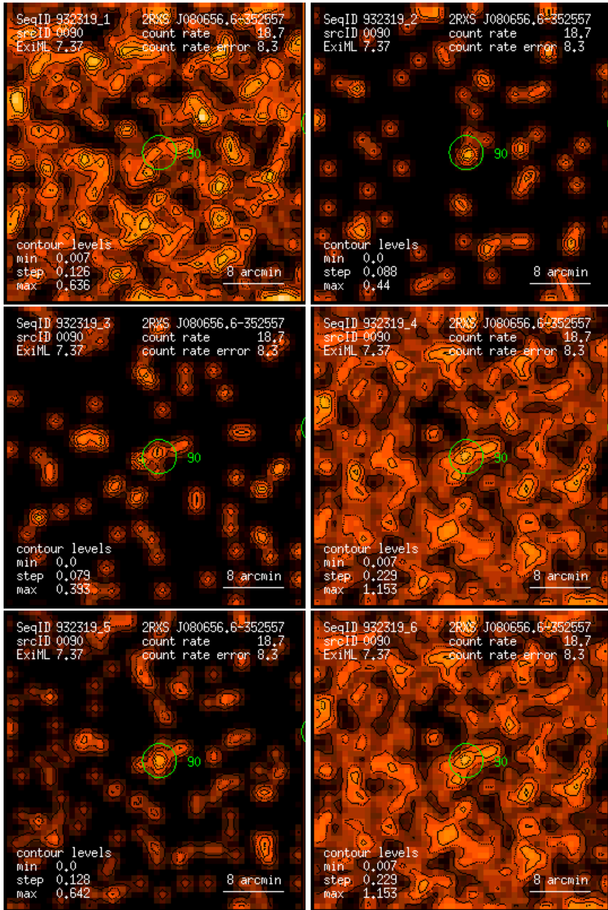
Figure 90: RASS 932319: detection 0090: band rate images, Gaussian filter: (1) PSPC channels 11 – 41, (2) 52 – 90, (3) 91 – 201, (4) 11 – 235, (5) 52 – 201, (6) 11 – 201. Broad band rates in counts/ks. Band rate contour levels in counts/ks/arcmin 2 .
