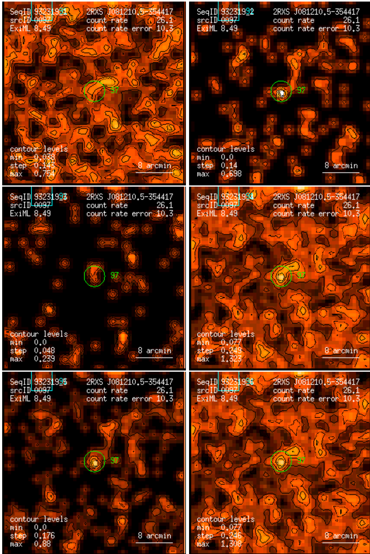
Figure 97: RASS 932319: detection 0097: band rate images, Gaussian filter: (1) PSPC channels 11 – 41, (2) 52 – 90, (3) 91 – 201, (4) 11 – 235, (5) 52 – 201, (6) 11 – 201. Broad band rates in counts/ks. Band rate contour levels in counts/ks/arcmin 2 .
