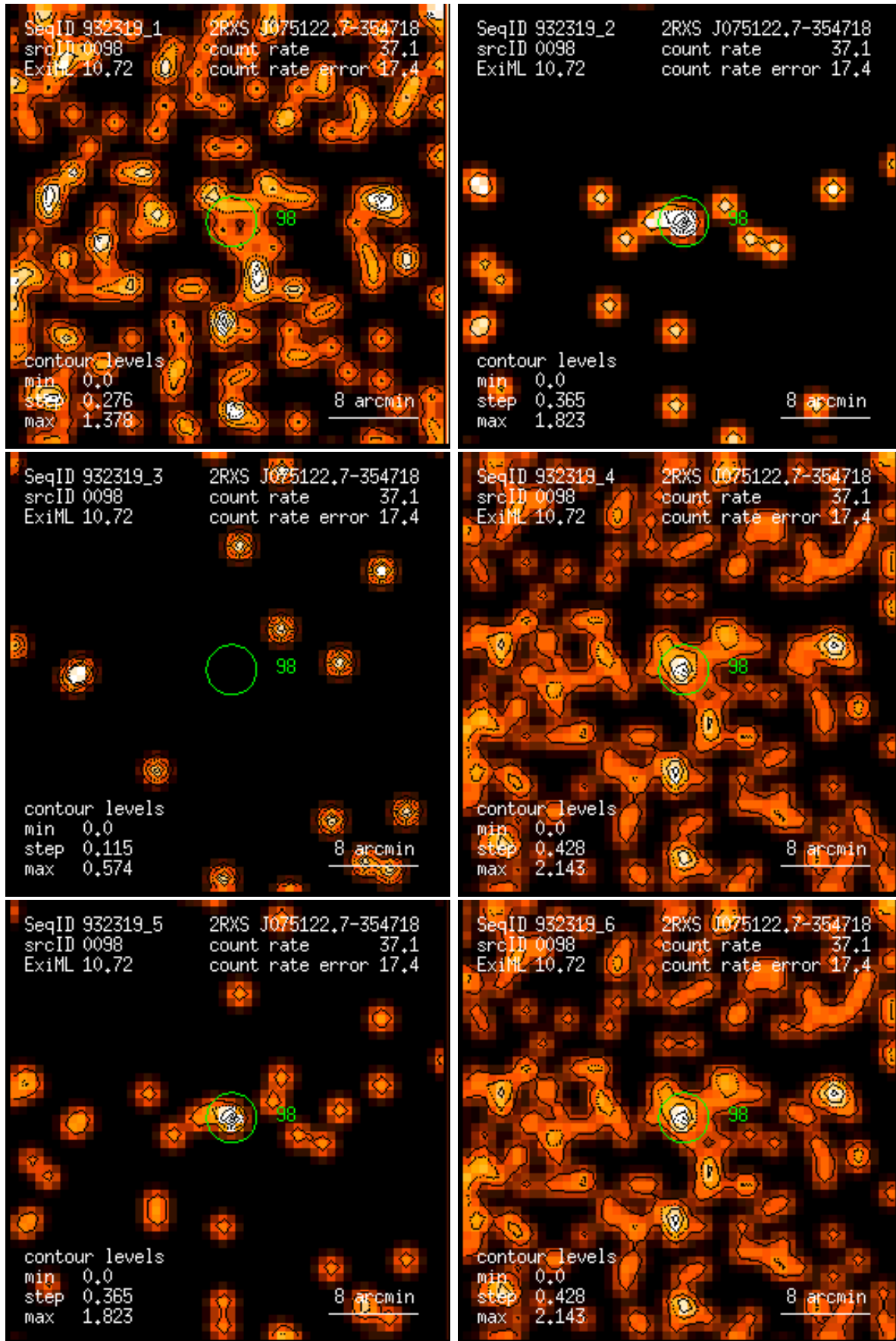
Figure 98: RASS 932319: detection 0098: band rate images, Gaussian filter: (1) PSPC channels 11 – 41, (2) 52 – 90, (3) 91 – 201, (4) 11 – 235, (5) 52 – 201, (6) 11 – 201. Broad band rates in counts/ks. Band rate contour levels in counts/ks/arcmin 2 .
