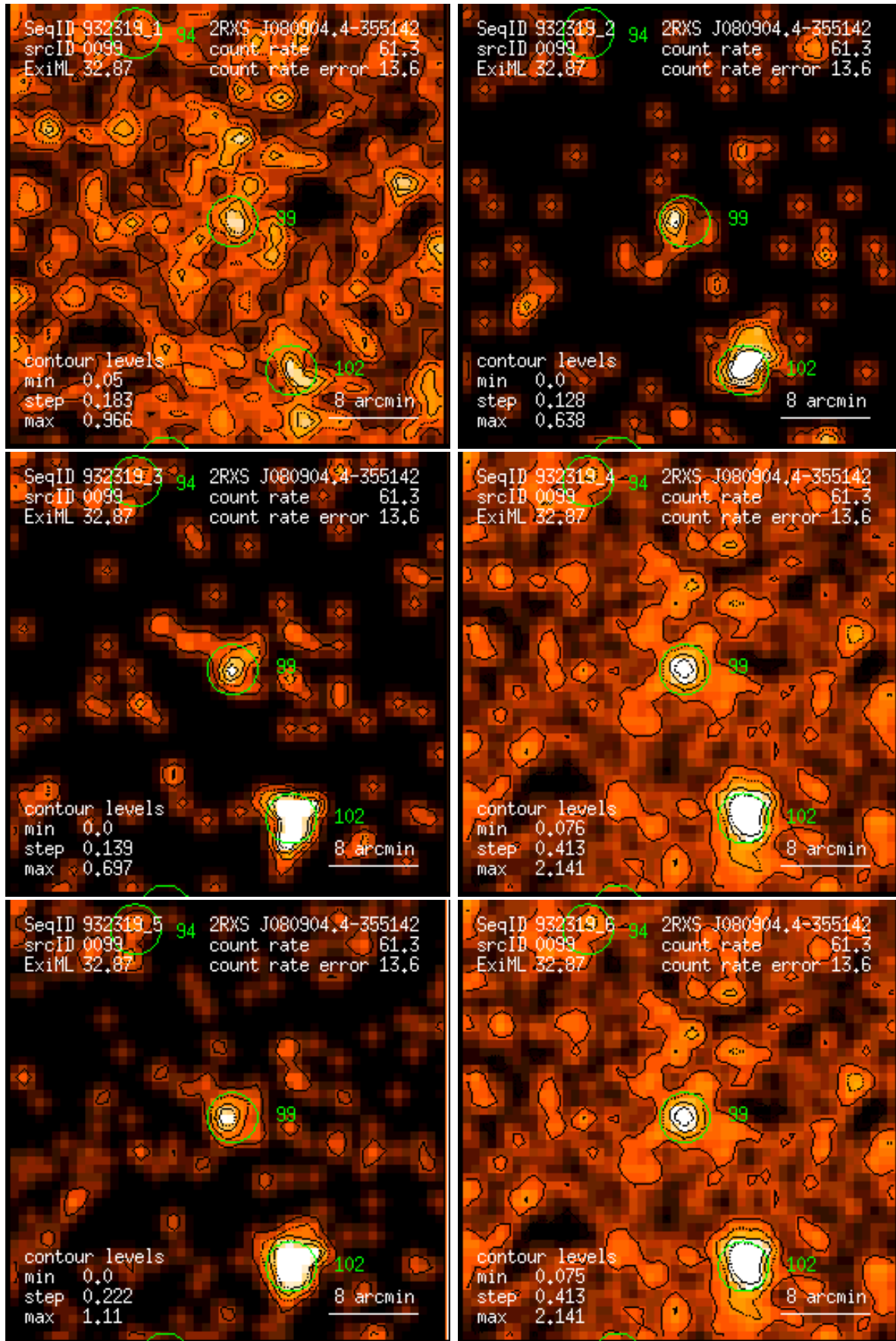
Figure 99: RASS 932319: detection 0099: band rate images, Gaussian filter: (1) PSPC channels 11 – 41, (2) 52 – 90, (3) 91 – 201, (4) 11 – 235, (5) 52 – 201, (6) 11 – 201. Broad band rates in counts/ks. Band rate contour levels in counts/ks/arcmin 2 .
