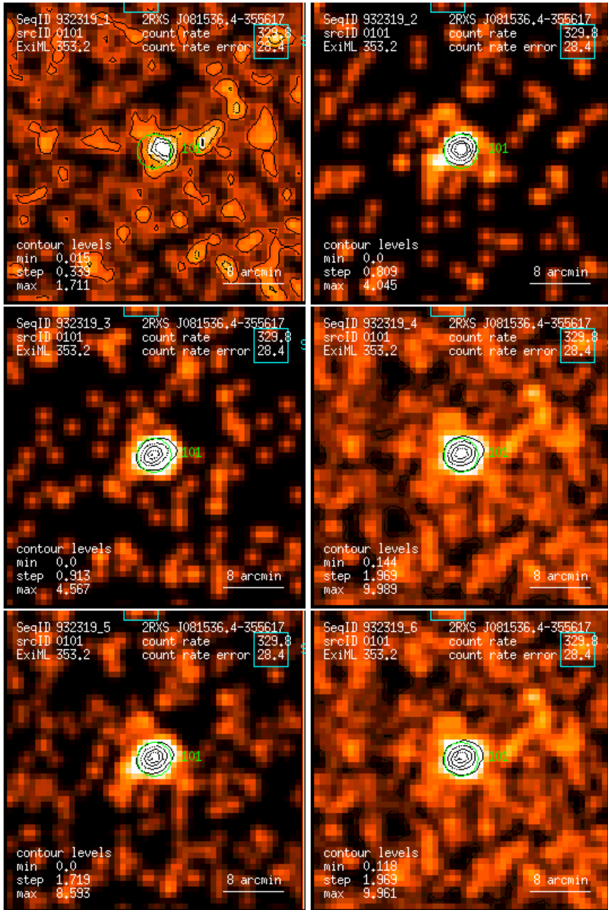
Figure 101: RASS 932319: detection 0101: band rate images, Gaussian filter: (1) PSPC channels 11 – 41, (2) 52 – 90, (3) 91 – 201, (4) 11 – 235, (5) 52 – 201, (6) 11 – 201. Broad band rates in counts/ks. Band rate contour levels in counts/ks/arcmin 2 .
