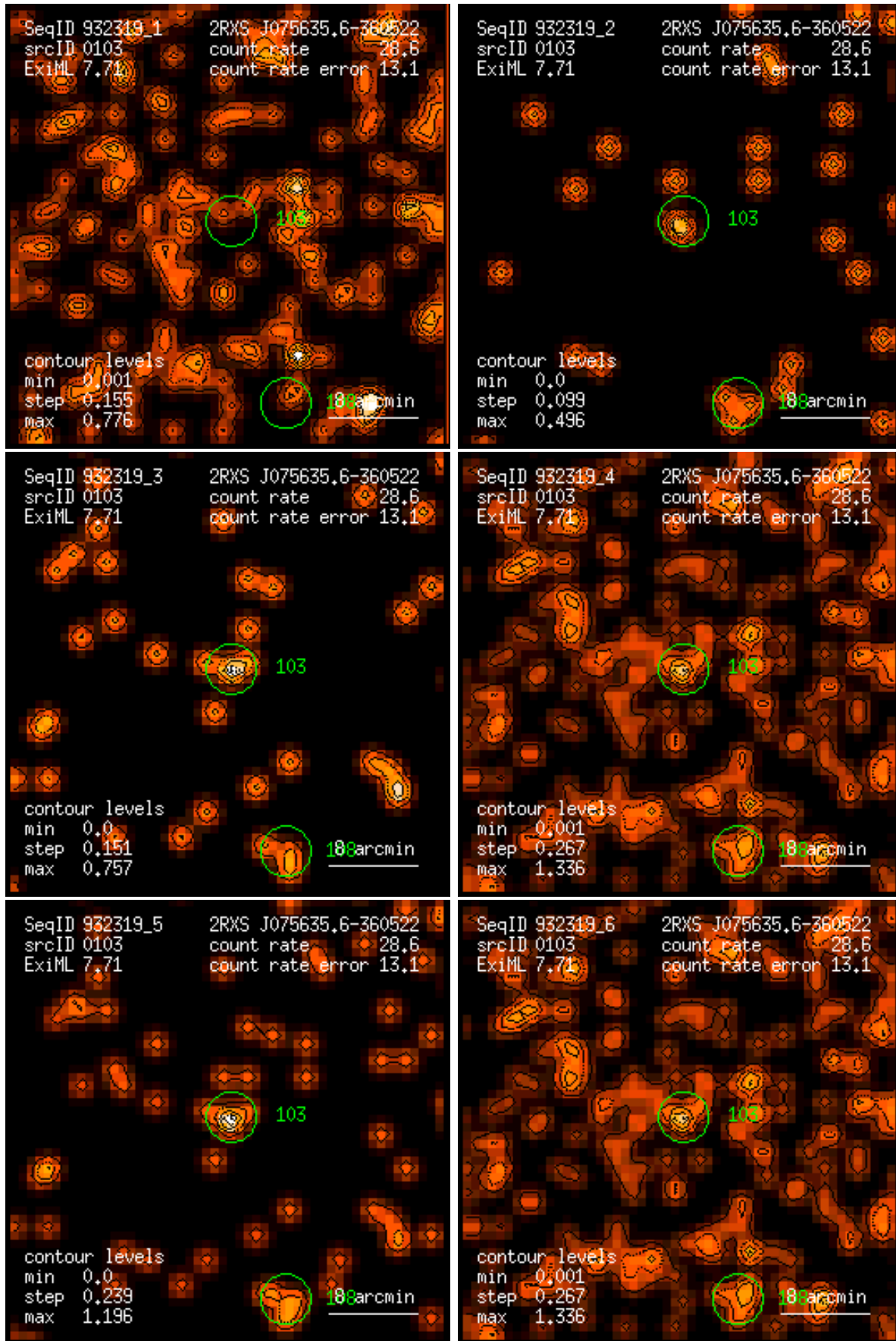
Figure 103: RASS 932319: detection 0103: band rate images, Gaussian filter: (1) PSPC channels 11 – 41, (2) 52 – 90, (3) 91 – 201, (4) 11 – 235, (5) 52 – 201, (6) 11 – 201. Broad band rates in counts/ks. Band rate contour levels in counts/ks/arcmin 2 .
