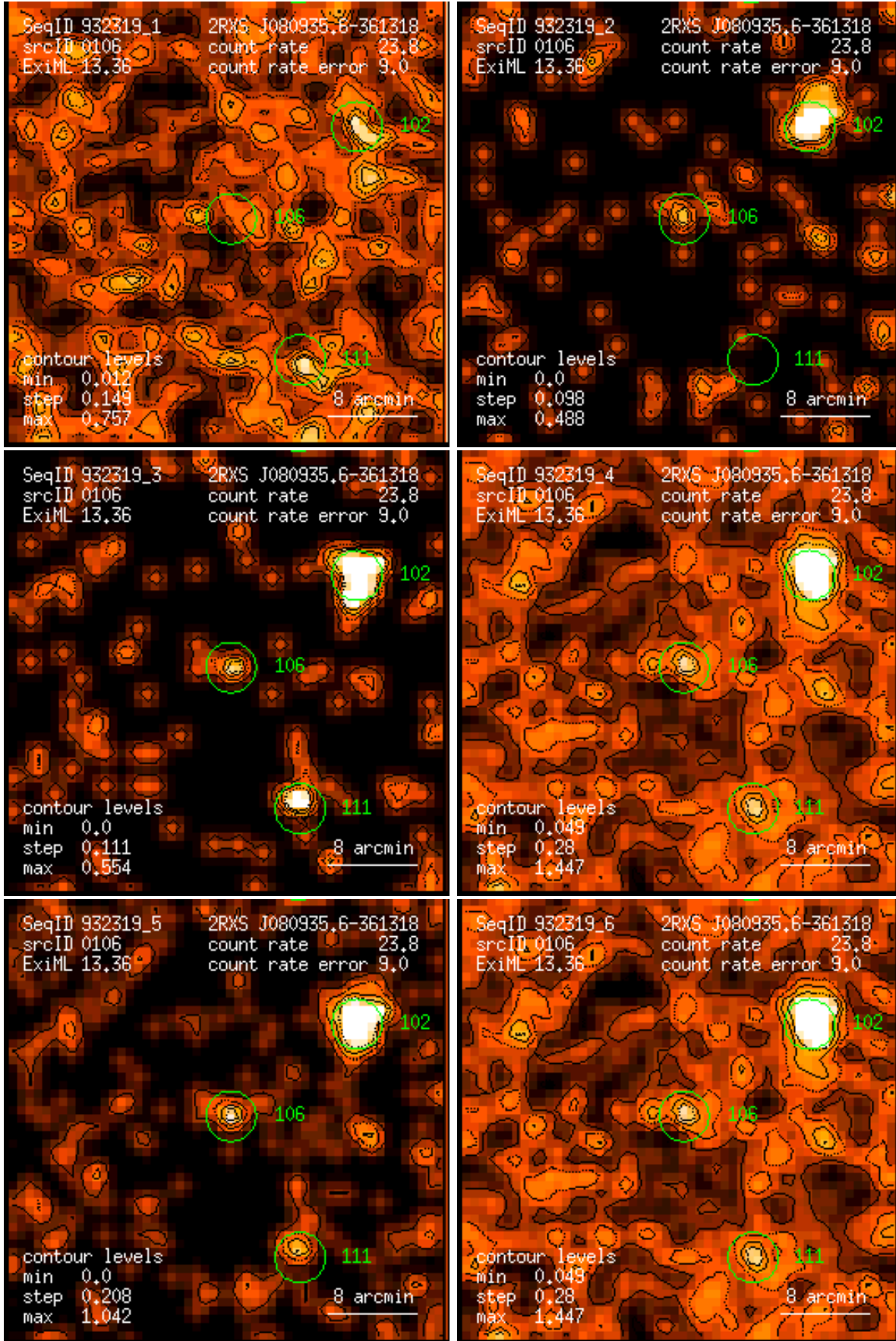
Figure 106: RASS 932319: detection 0106: band rate images, Gaussian filter: (1) PSPC channels 11 – 41, (2) 52 – 90, (3) 91 – 201, (4) 11 – 235, (5) 52 – 201, (6) 11 – 201. Broad band rates in counts/ks. Band rate contour levels in counts/ks/arcmin 2 .
