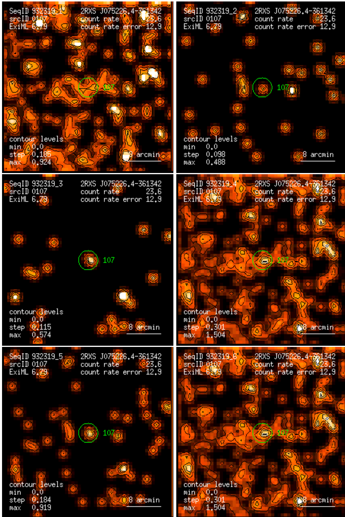
Figure 107: RASS 932319: detection 0107: band rate images, Gaussian filter: (1) PSPC channels 11 – 41, (2) 52 – 90, (3) 91 – 201, (4) 11 – 235, (5) 52 – 201, (6) 11 – 201. Broad band rates in counts/ks. Band rate contour levels in counts/ks/arcmin 2 .
