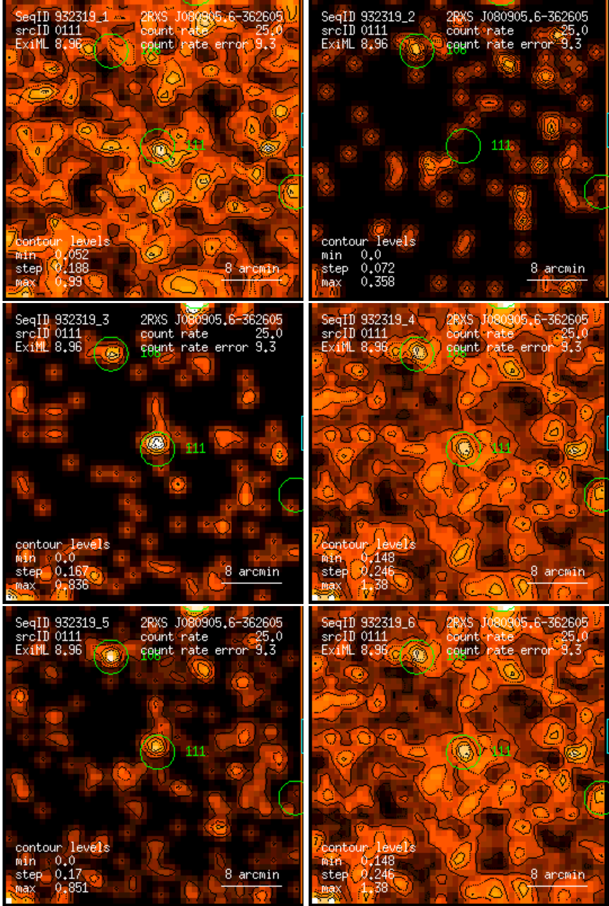
Figure 111: RASS 932319: detection 0111: band rate images, Gaussian filter: (1) PSPC channels 11 – 41, (2) 52 – 90, (3) 91 – 201, (4) 11 – 235, (5) 52 – 201, (6) 11 – 201. Broad band rates in counts/ks. Band rate contour levels in counts/ks/arcmin 2 .
