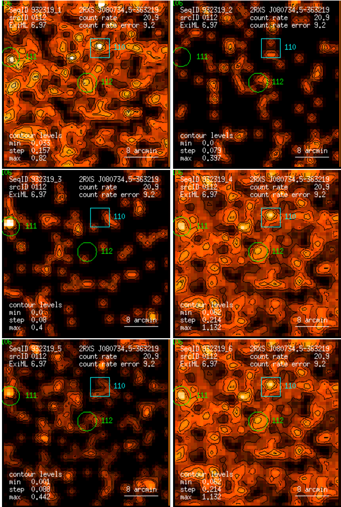
Figure 112: RASS 932319: detection 0112: band rate images, Gaussian filter: (1) PSPC channels 11 – 41, (2) 52 – 90, (3) 91 – 201, (4) 11 – 235, (5) 52 – 201, (6) 11 – 201. Broad band rates in counts/ks. Band rate contour levels in counts/ks/arcmin 2 .
