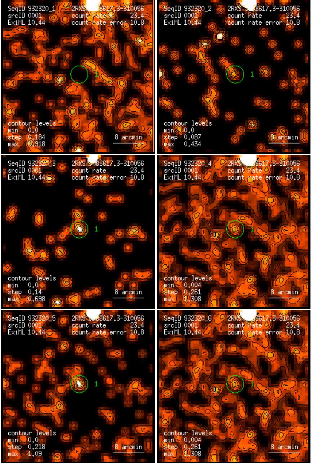
Figure 1: RASS 932320: detection 0001: band rate images, Gaussian filter: (1) PSPC channels 11 – 41, (2) 52 – 90, (3) 91 – 201, (4) 11 – 235, (5) 52 – 201, (6) 11 – 201. Broad band rates in counts/ks. Band rate contour levels in counts/ks/arcmin 2 .
