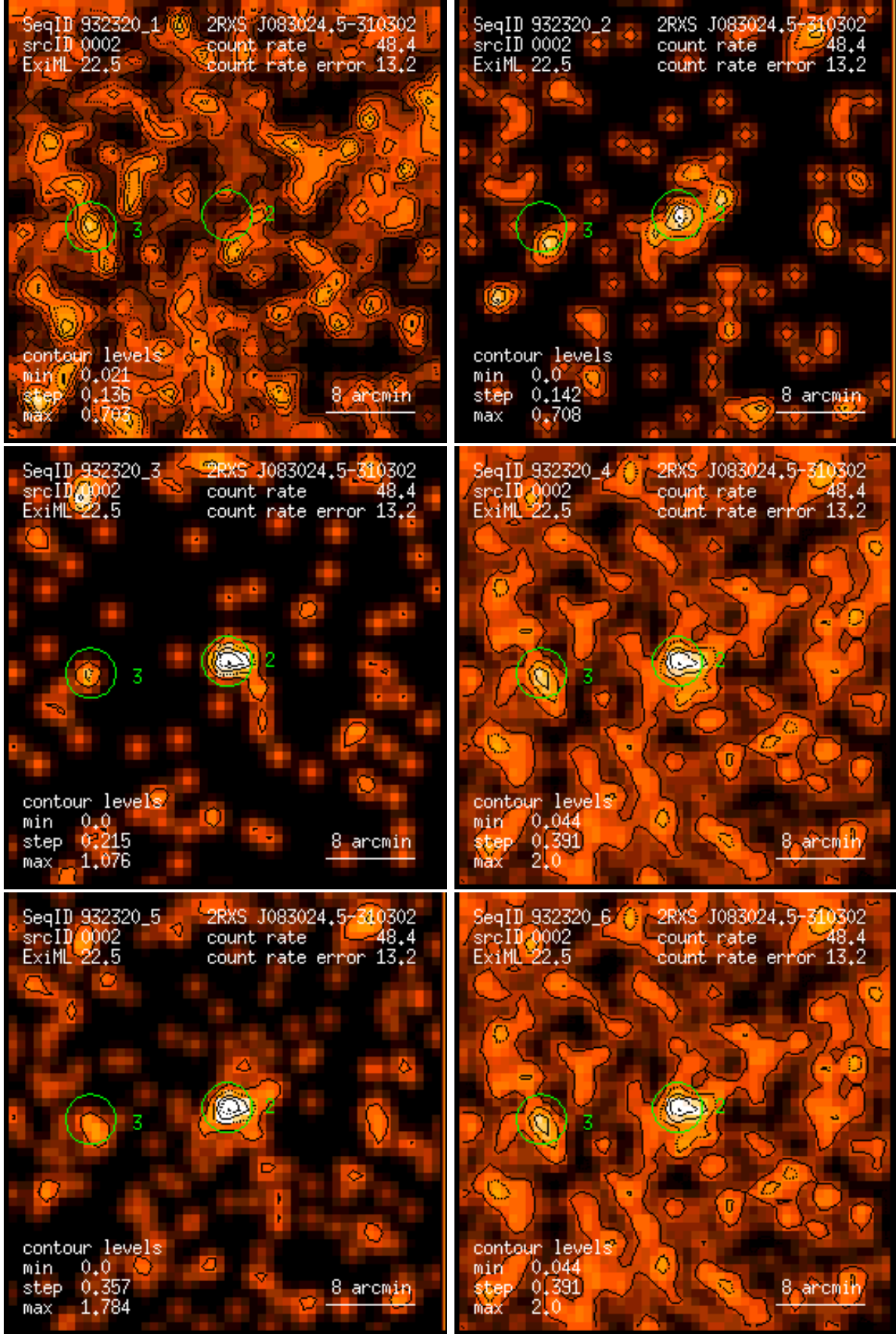
Figure 2: RASS 932320: detection 0002: band rate images, Gaussian filter: (1) PSPC channels 11 – 41, (2) 52 – 90, (3) 91 – 201, (4) 11 – 235, (5) 52 – 201, (6) 11 – 201. Broad band rates in counts/ks. Band rate contour levels in counts/ks/arcmin 2 .
