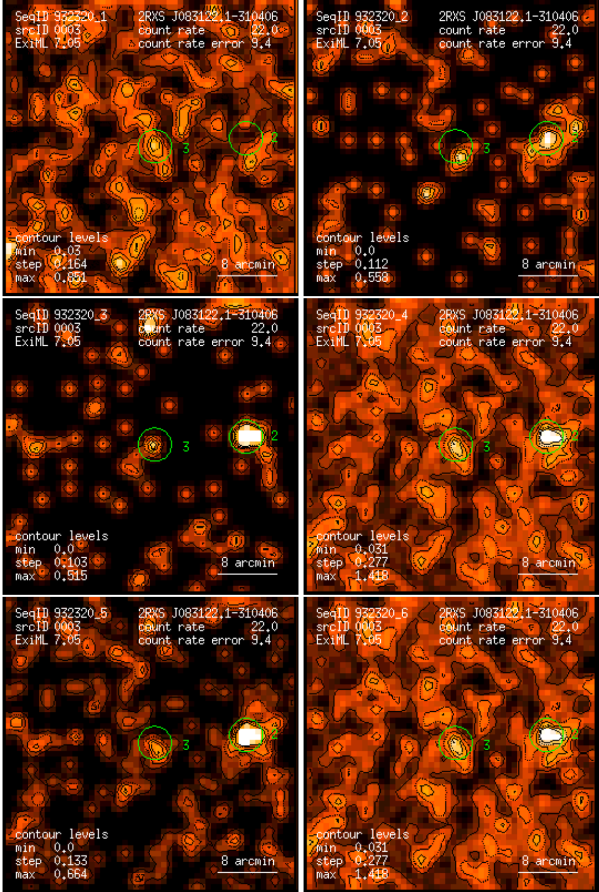
Figure 3: RASS 932320: detection 0003: band rate images, Gaussian filter: (1) PSPC channels 11 – 41, (2) 52 – 90, (3) 91 – 201, (4) 11 – 235, (5) 52 – 201, (6) 11 – 201. Broad band rates in counts/ks. Band rate contour levels in counts/ks/arcmin 2 .
