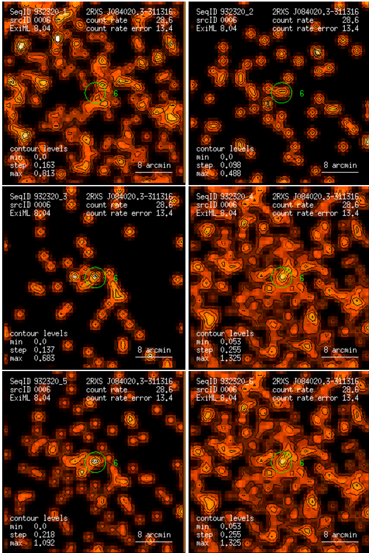
Figure 6: RASS 932320: detection 0006: band rate images, Gaussian filter: (1) PSPC channels 11 – 41, (2) 52 – 90, (3) 91 – 201, (4) 11 – 235, (5) 52 – 201, (6) 11 – 201. Broad band rates in counts/ks. Band rate contour levels in counts/ks/arcmin 2 .
