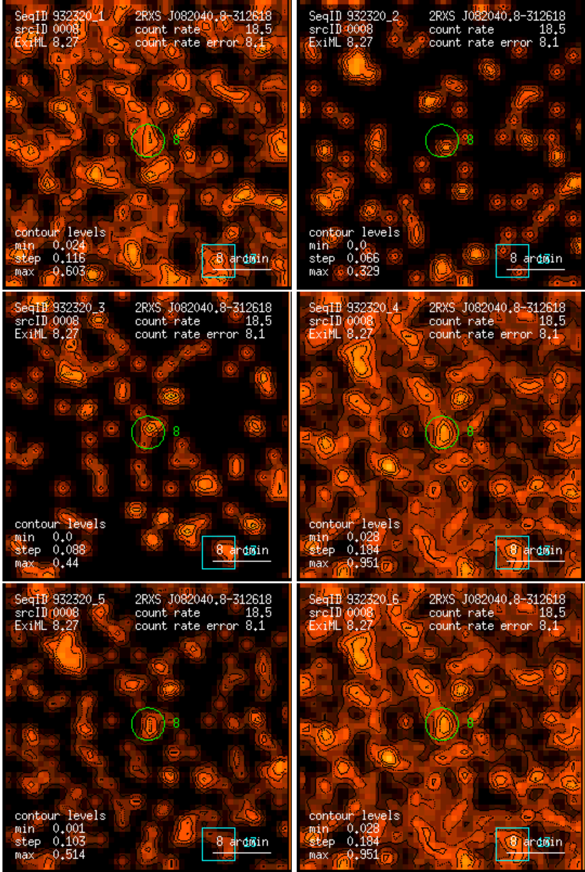
Figure 8: RASS 932320: detection 0008: band rate images, Gaussian filter: (1) PSPC channels 11 – 41, (2) 52 – 90, (3) 91 – 201, (4) 11 – 235, (5) 52 – 201, (6) 11 – 201. Broad band rates in counts/ks. Band rate contour levels in counts/ks/arcmin 2 .
