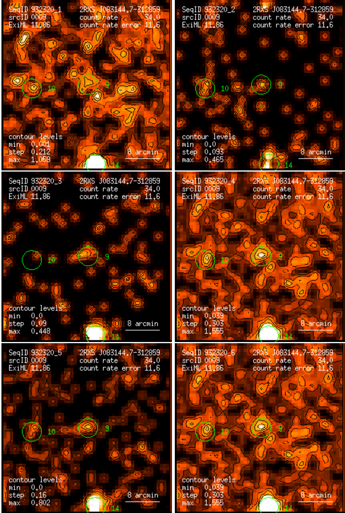
Figure 9: RASS 932320: detection 0009: band rate images, Gaussian filter: (1) PSPC channels 11 – 41, (2) 52 – 90, (3) 91 – 201, (4) 11 – 235, (5) 52 – 201, (6) 11 – 201. Broad band rates in counts/ks. Band rate contour levels in counts/ks/arcmin 2 .
