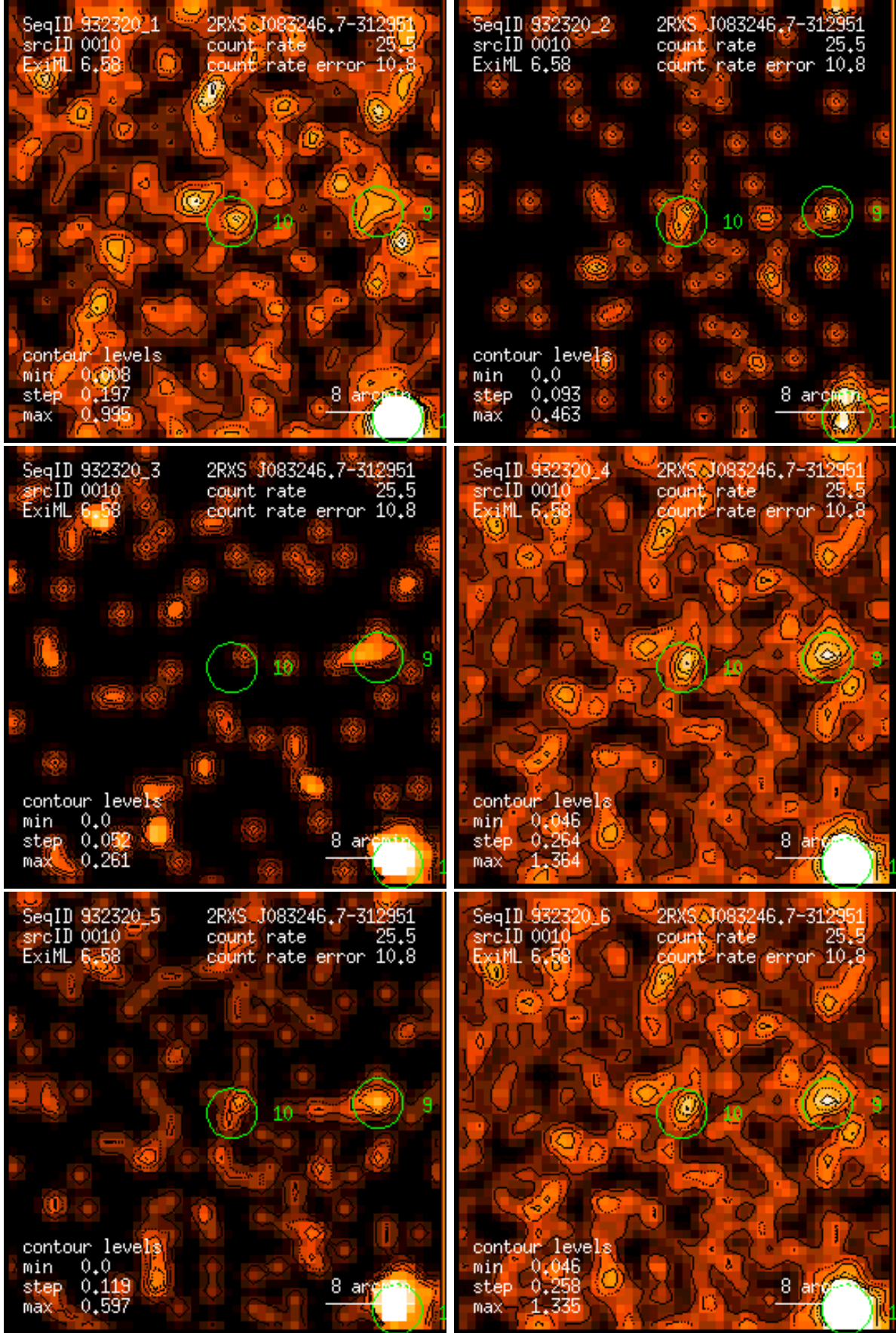
Figure 10: RASS 932320: detection 0010: band rate images, Gaussian filter: (1) PSPC channels 11 – 41, (2) 52 – 90, (3) 91 – 201, (4) 11 – 235, (5) 52 – 201, (6) 11 – 201. Broad band rates in counts/ks. Band rate contour levels in counts/ks/arcmin 2 .
