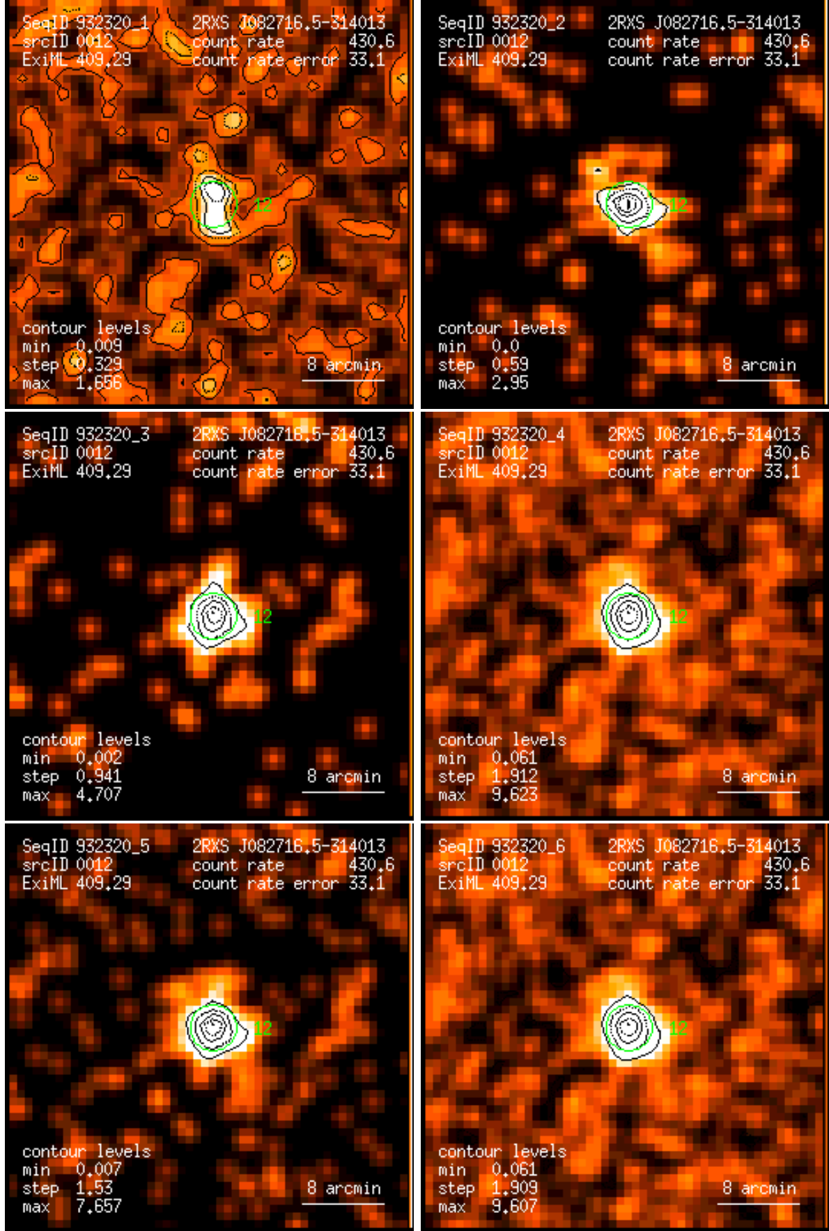
Figure 12: RASS 932320: detection 0012: band rate images, Gaussian filter: (1) PSPC channels 11 – 41, (2) 52 – 90, (3) 91 – 201, (4) 11 – 235, (5) 52 – 201, (6) 11 – 201. Broad band rates in counts/ks. Band rate contour levels in counts/ks/arcmin 2 .
