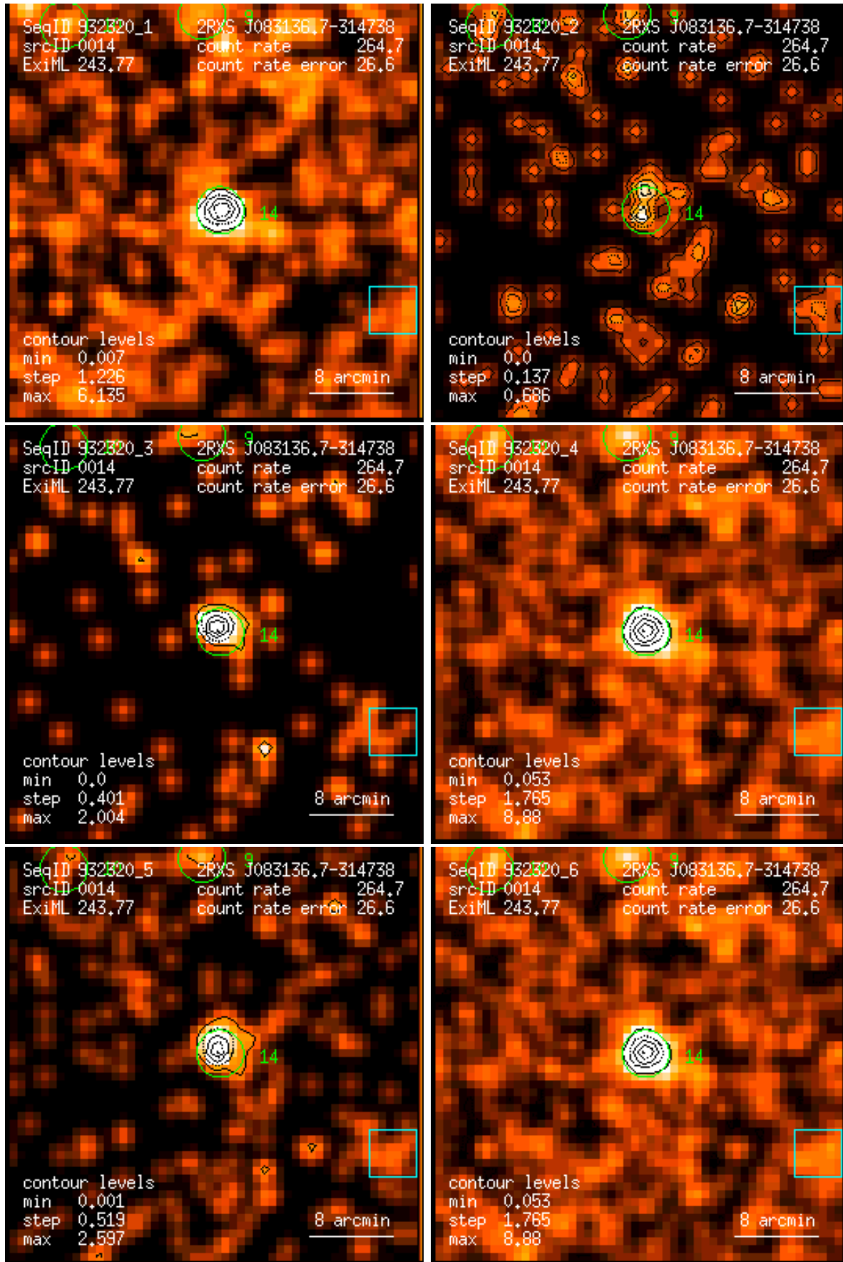
Figure 14: RASS 932320: detection 0014: band rate images, Gaussian filter: (1) PSPC channels 11 – 41, (2) 52 – 90, (3) 91 – 201, (4) 11 – 235, (5) 52 – 201, (6) 11 – 201. Broad band rates in counts/ks. Band rate contour levels in counts/ks/arcmin 2 .
