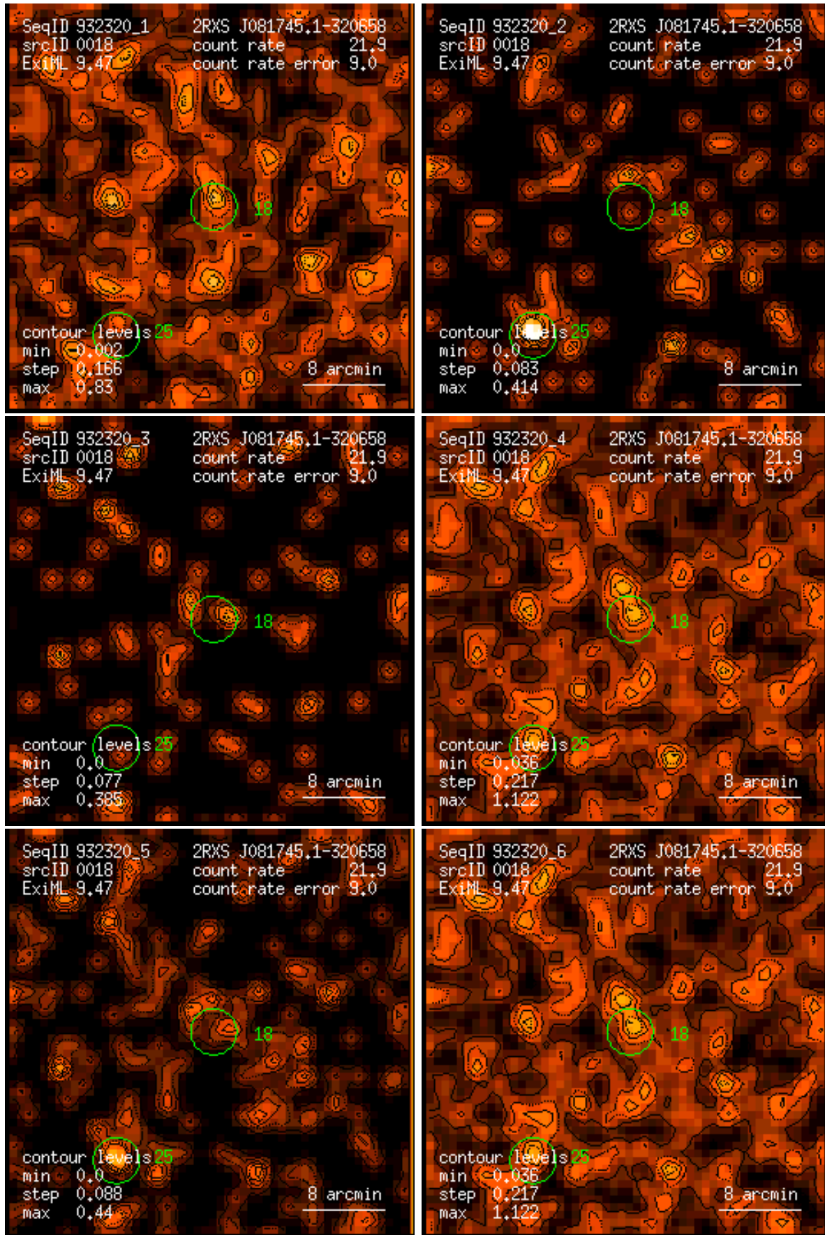
Figure 18: RASS 932320: detection 0018: band rate images, Gaussian filter: (1) PSPC channels 11 – 41, (2) 52 – 90, (3) 91 – 201, (4) 11 – 235, (5) 52 – 201, (6) 11 – 201. Broad band rates in counts/ks. Band rate contour levels in counts/ks/arcmin 2 .
