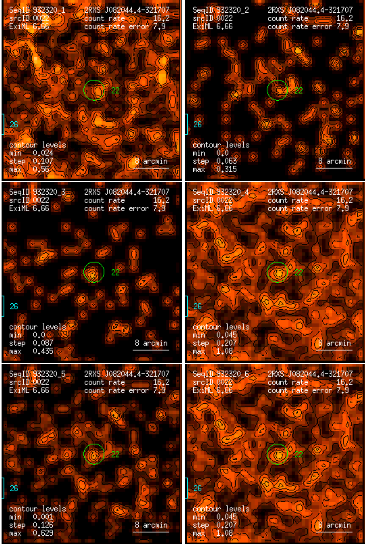
Figure 22: RASS 932320: detection 0022: band rate images, Gaussian filter: (1) PSPC channels 11 – 41, (2) 52 – 90, (3) 91 – 201, (4) 11 – 235, (5) 52 – 201, (6) 11 – 201. Broad band rates in counts/ks. Band rate contour levels in counts/ks/arcmin 2 .
