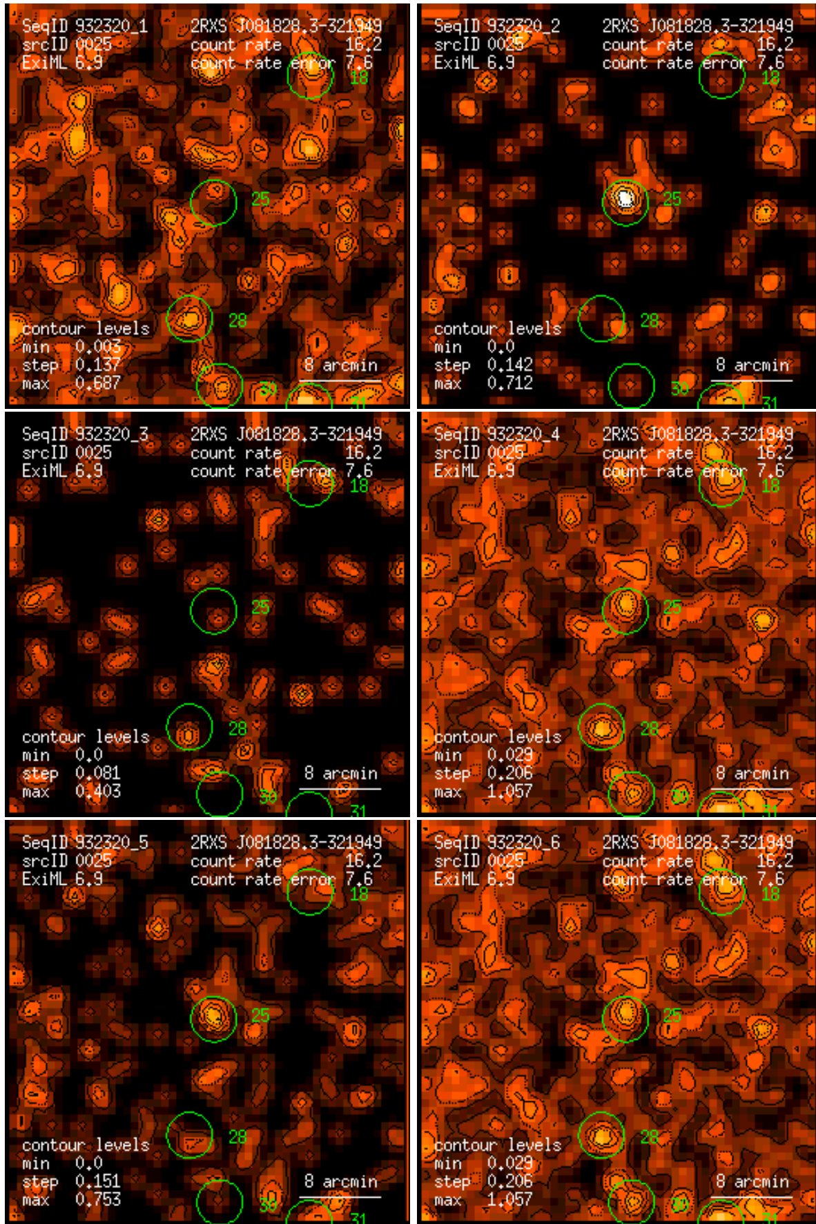
Figure 25: RASS 932320: detection 0025: band rate images, Gaussian filter: (1) PSPC channels 11 – 41, (2) 52 – 90, (3) 91 – 201, (4) 11 – 235, (5) 52 – 201, (6) 11 – 201. Broad band rates in counts/ks. Band rate contour levels in counts/ks/arcmin 2 .
