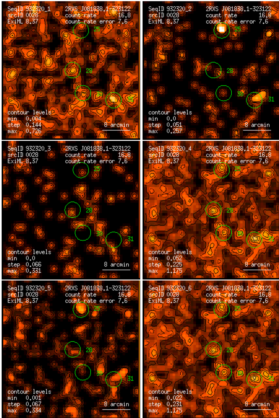
Figure 28: RASS 932320: detection 0028: band rate images, Gaussian filter: (1) PSPC channels 11 – 41, (2) 52 – 90, (3) 91 – 201, (4) 11 – 235, (5) 52 – 201, (6) 11 – 201. Broad band rates in counts/ks. Band rate contour levels in counts/ks/arcmin 2 .
