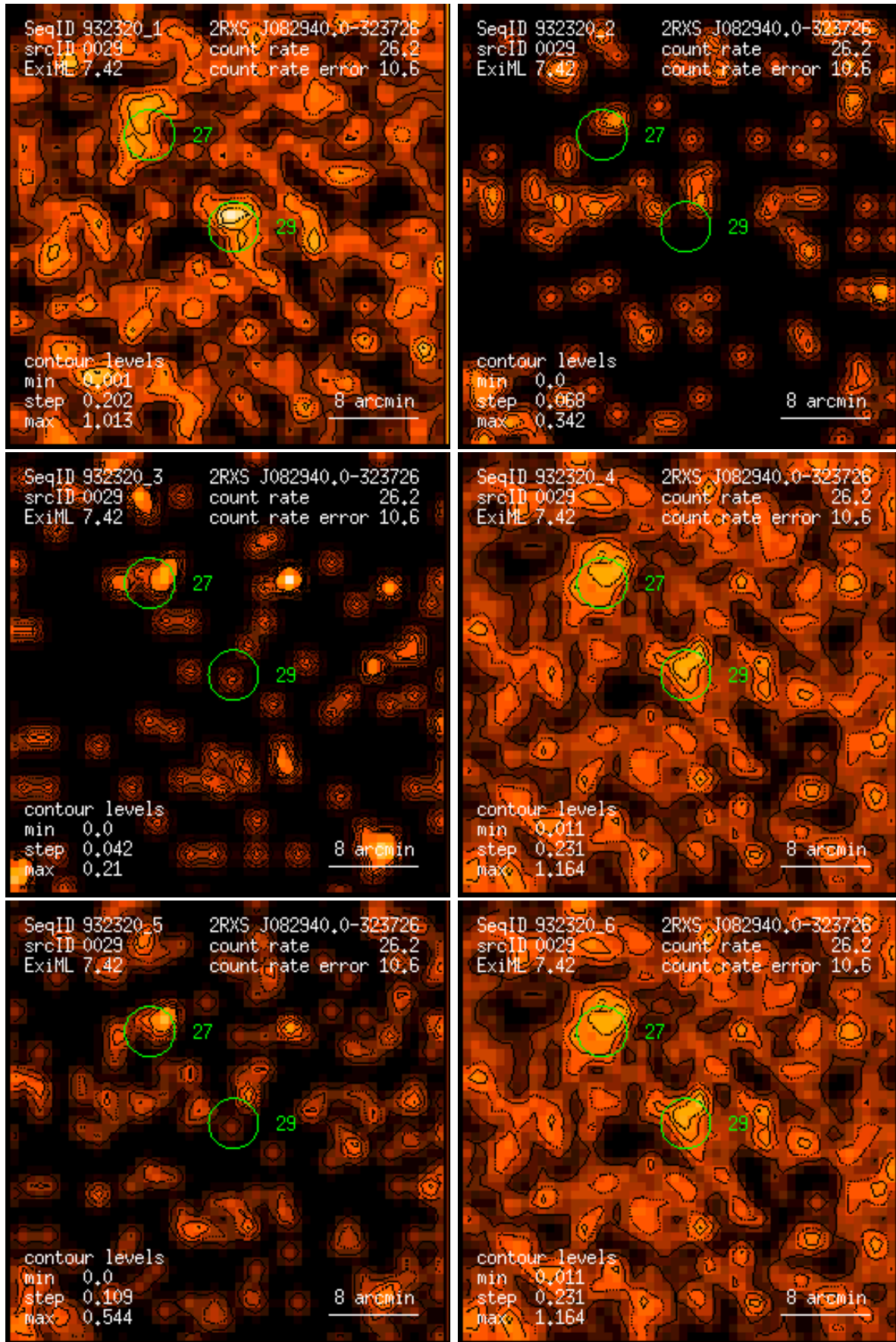
Figure 29: RASS 932320: detection 0029: band rate images, Gaussian filter: (1) PSPC channels 11 – 41, (2) 52 – 90, (3) 91 – 201, (4) 11 – 235, (5) 52 – 201, (6) 11 – 201. Broad band rates in counts/ks. Band rate contour levels in counts/ks/arcmin 2 .
