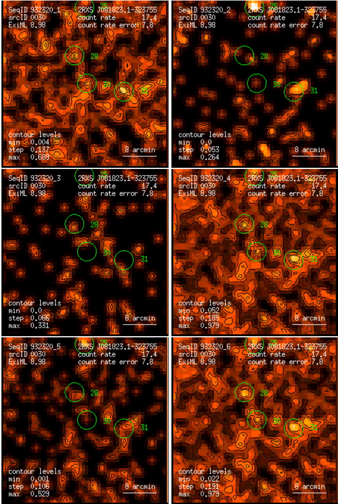
Figure 30: RASS 932320: detection 0030: band rate images, Gaussian filter: (1) PSPC channels 11 – 41, (2) 52 – 90, (3) 91 – 201, (4) 11 – 235, (5) 52 – 201, (6) 11 – 201. Broad band rates in counts/ks. Band rate contour levels in counts/ks/arcmin 2 .
