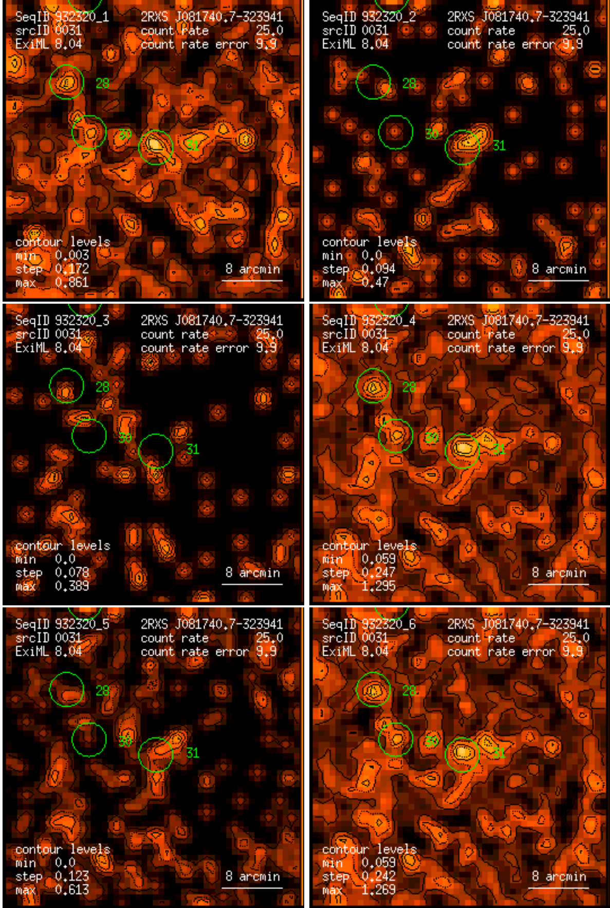
Figure 31: RASS 932320: detection 0031: band rate images, Gaussian filter: (1) PSPC channels 11 – 41, (2) 52 – 90, (3) 91 – 201, (4) 11 – 235, (5) 52 – 201, (6) 11 – 201. Broad band rates in counts/ks. Band rate contour levels in counts/ks/arcmin 2 .
