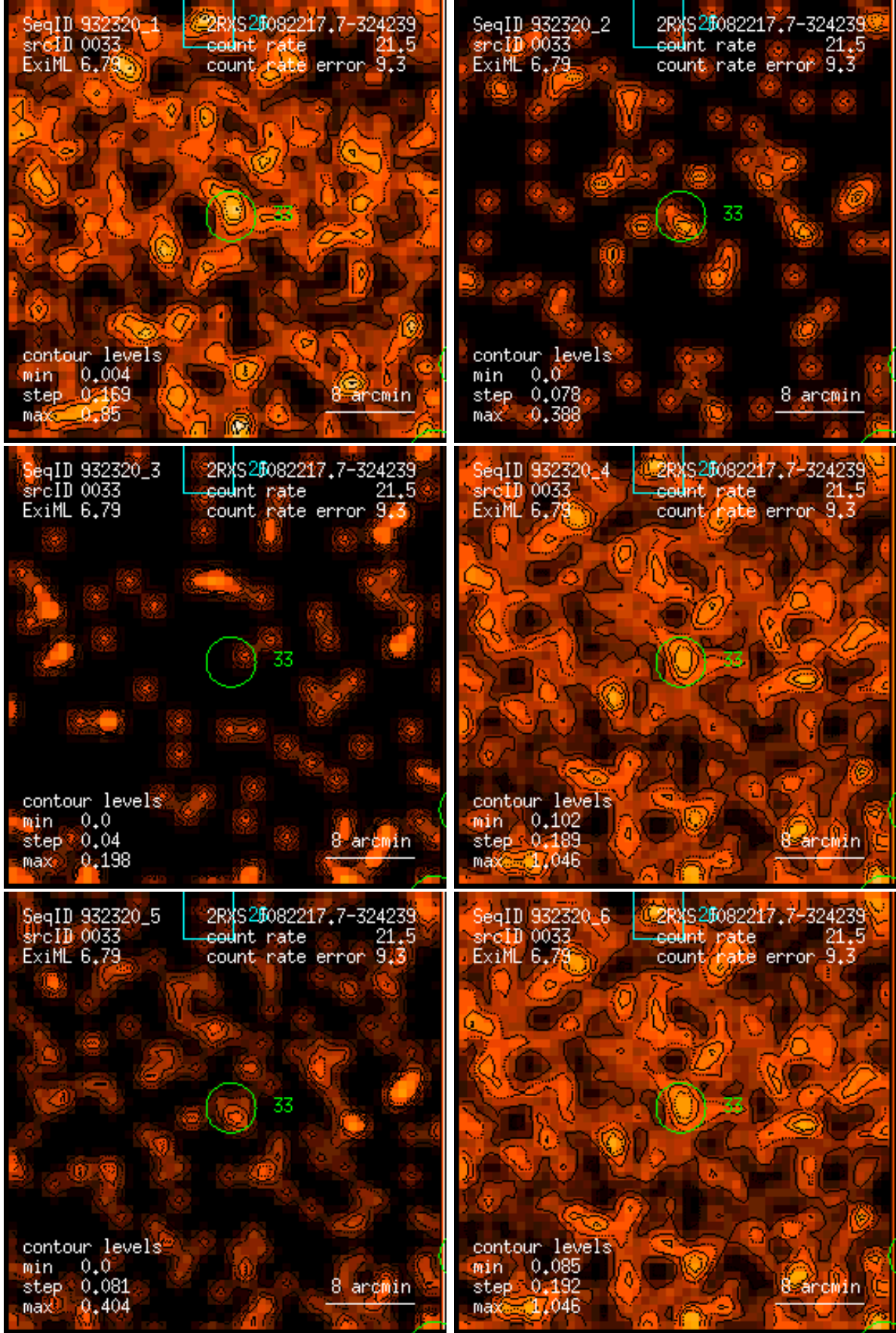
Figure 33: RASS 932320: detection 0033: band rate images, Gaussian filter: (1) PSPC channels 11 – 41, (2) 52 – 90, (3) 91 – 201, (4) 11 – 235, (5) 52 – 201, (6) 11 – 201. Broad band rates in counts/ks. Band rate contour levels in counts/ks/arcmin 2 .
