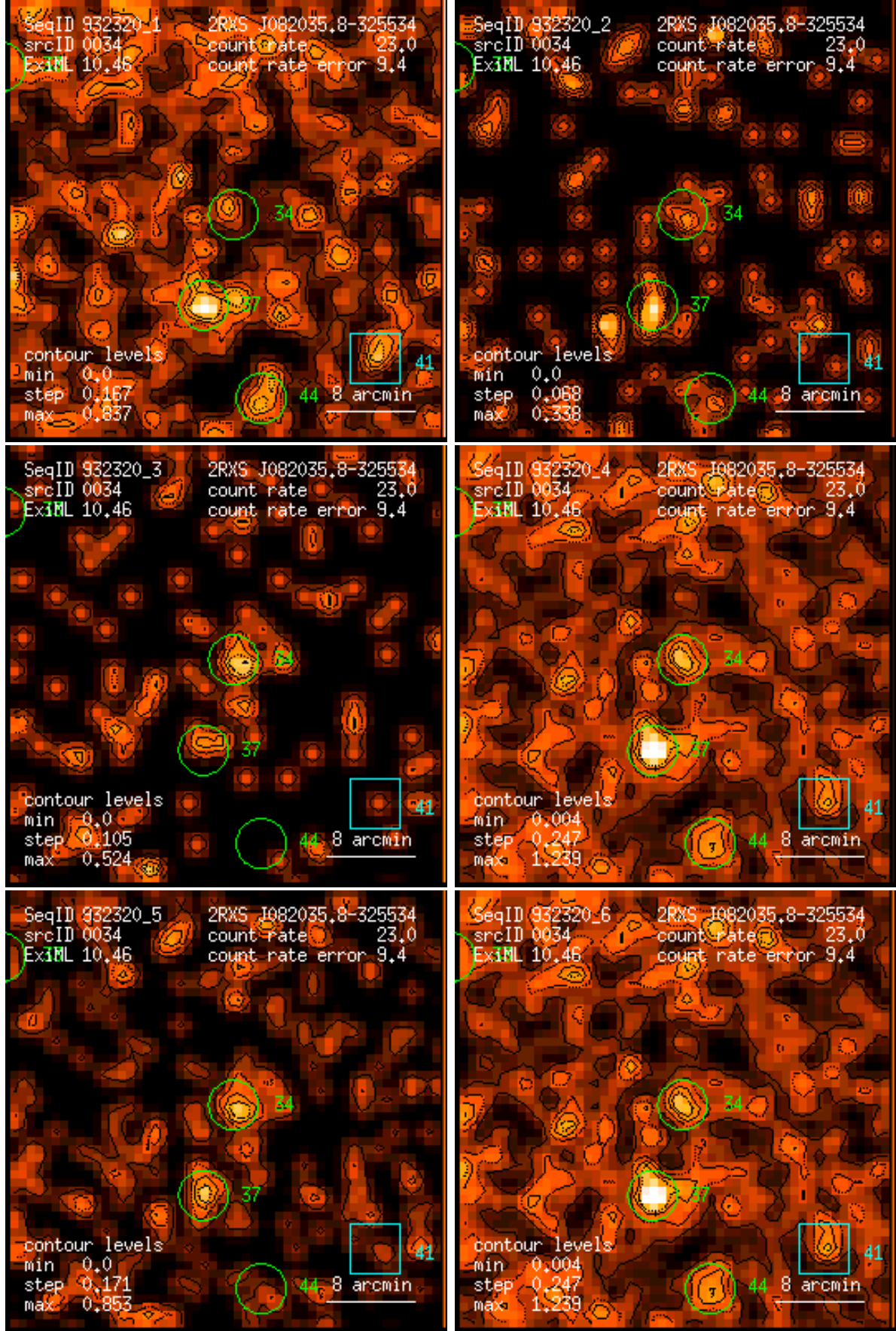
Figure 34: RASS 932320: detection 0034: band rate images, Gaussian filter: (1) PSPC channels 11 – 41, (2) 52 – 90, (3) 91 – 201, (4) 11 – 235, (5) 52 – 201, (6) 11 – 201. Broad band rates in counts/ks. Band rate contour levels in counts/ks/arcmin 2 .
