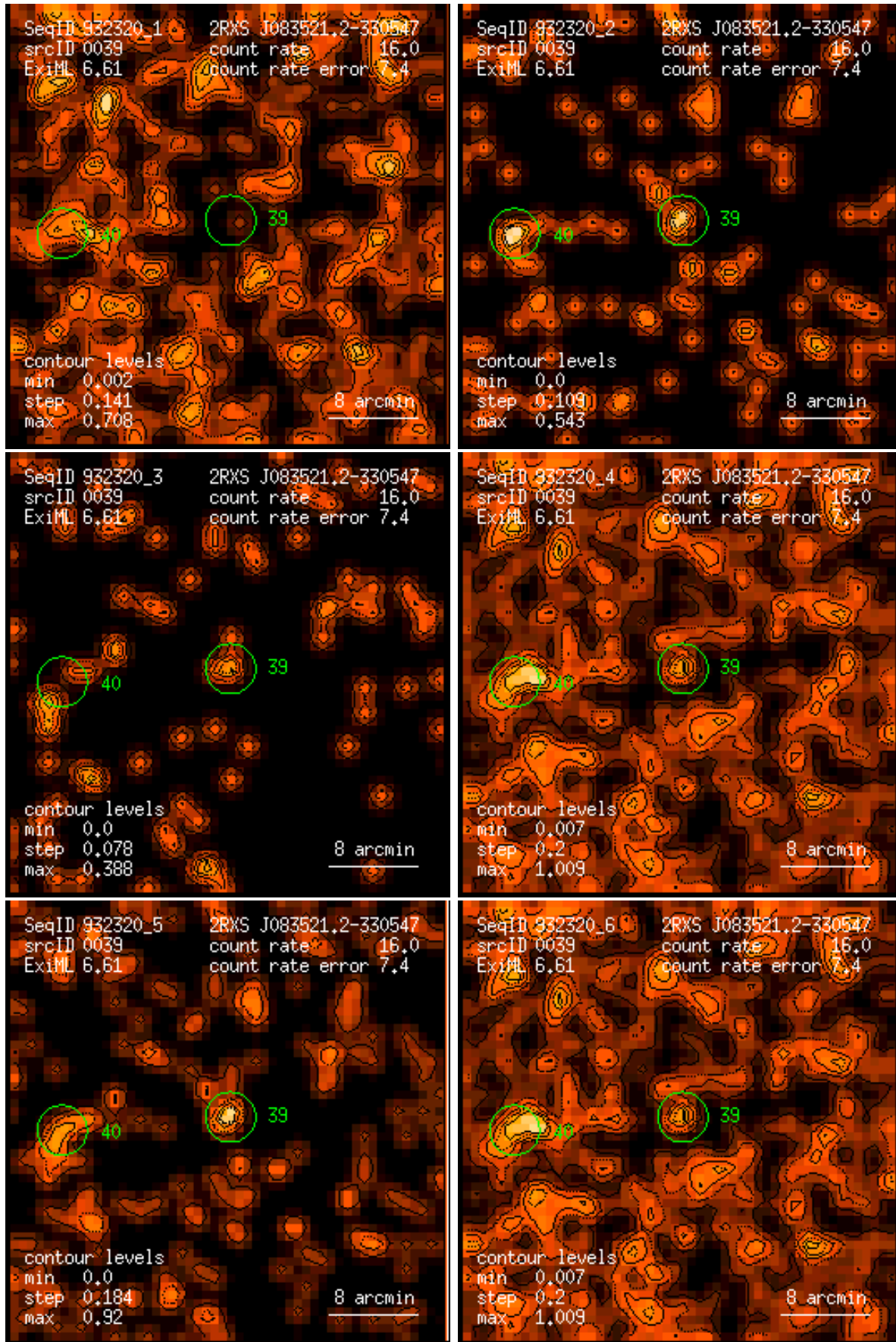
Figure 39: RASS 932320: detection 0039: band rate images, Gaussian filter: (1) PSPC channels 11 – 41, (2) 52 – 90, (3) 91 – 201, (4) 11 – 235, (5) 52 – 201, (6) 11 – 201. Broad band rates in counts/ks. Band rate contour levels in counts/ks/arcmin 2 .
