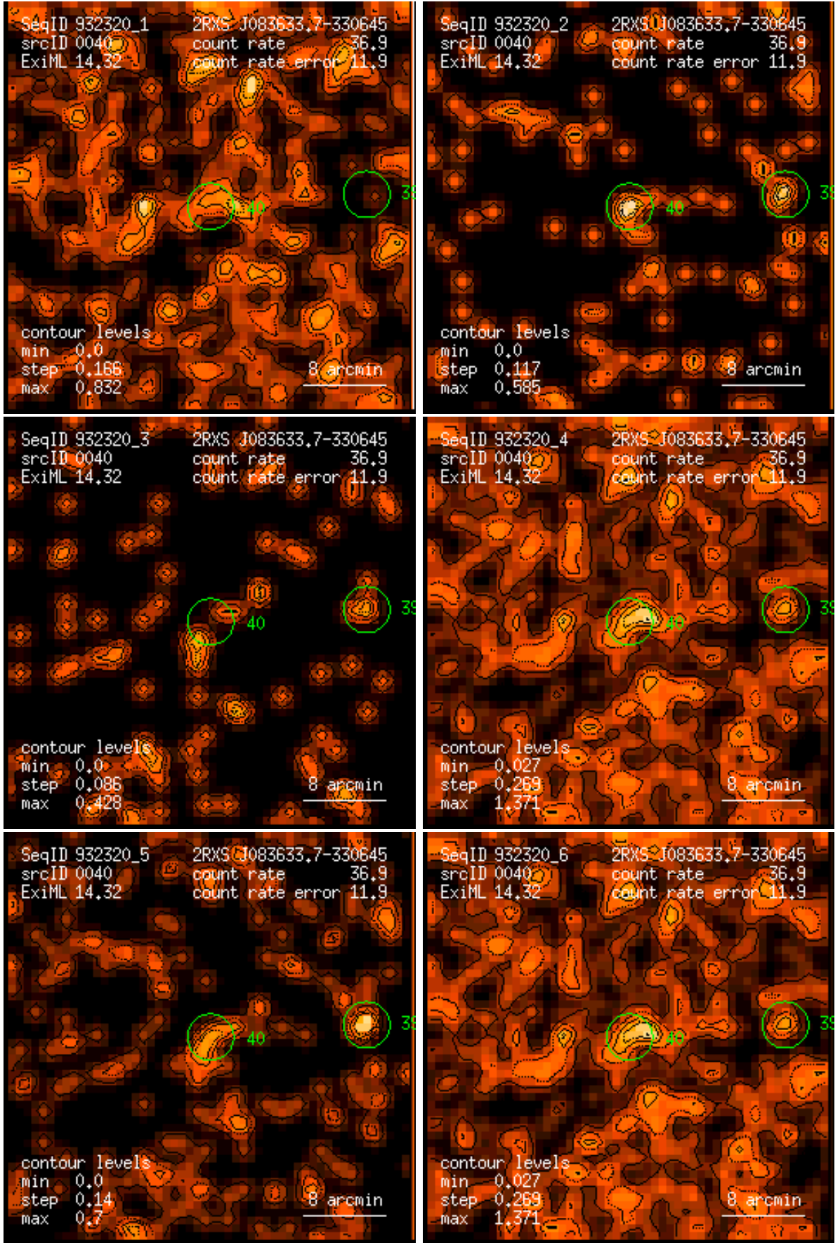
Figure 40: RASS 932320: detection 0040: band rate images, Gaussian filter: (1) PSPC channels 11 – 41, (2) 52 – 90, (3) 91 – 201, (4) 11 – 235, (5) 52 – 201, (6) 11 – 201. Broad band rates in counts/ks. Band rate contour levels in counts/ks/arcmin 2 .
