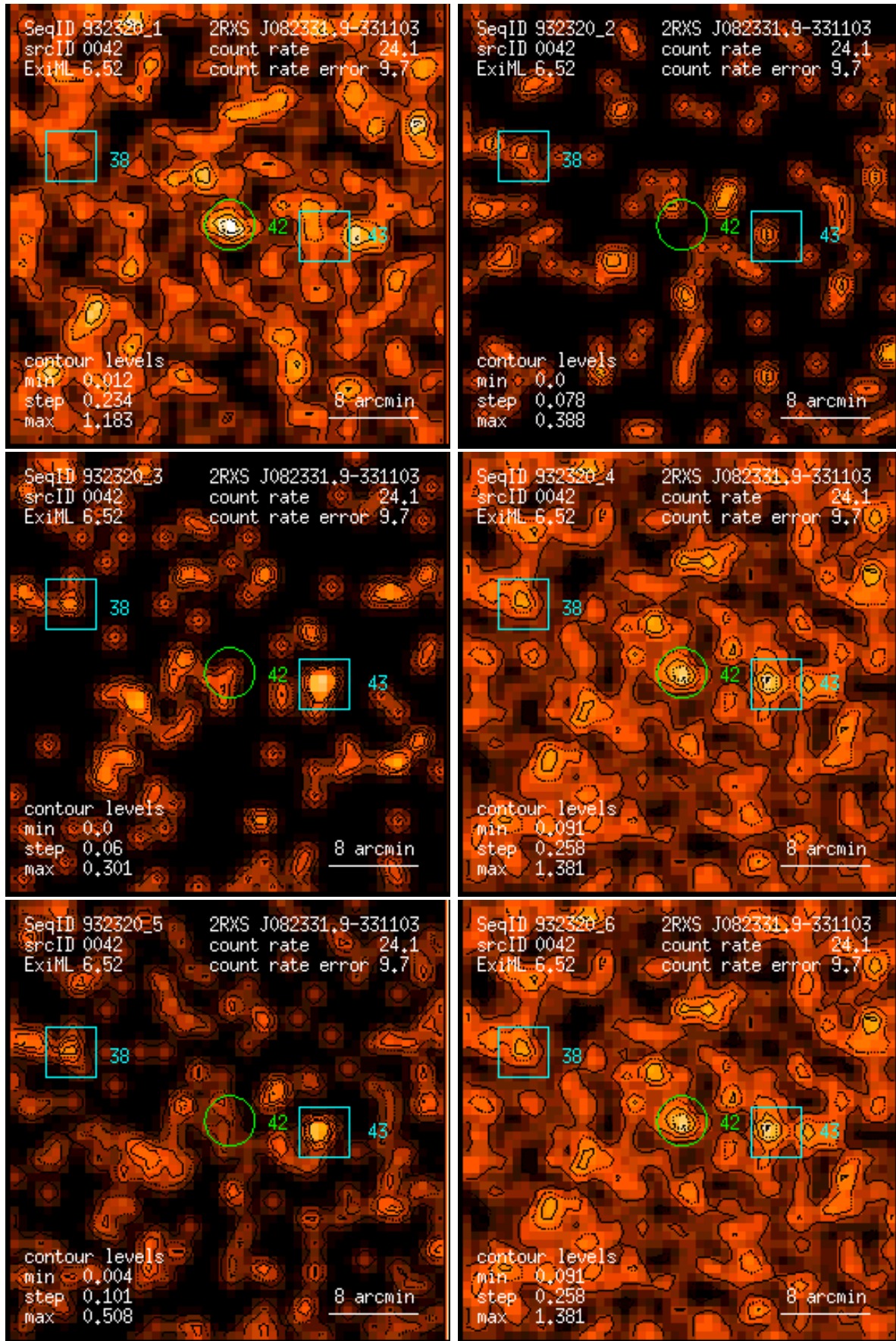
Figure 42: RASS 932320: detection 0042: band rate images, Gaussian filter: (1) PSPC channels 11 – 41, (2) 52 – 90, (3) 91 – 201, (4) 11 – 235, (5) 52 – 201, (6) 11 – 201. Broad band rates in counts/ks. Band rate contour levels in counts/ks/arcmin 2 .
